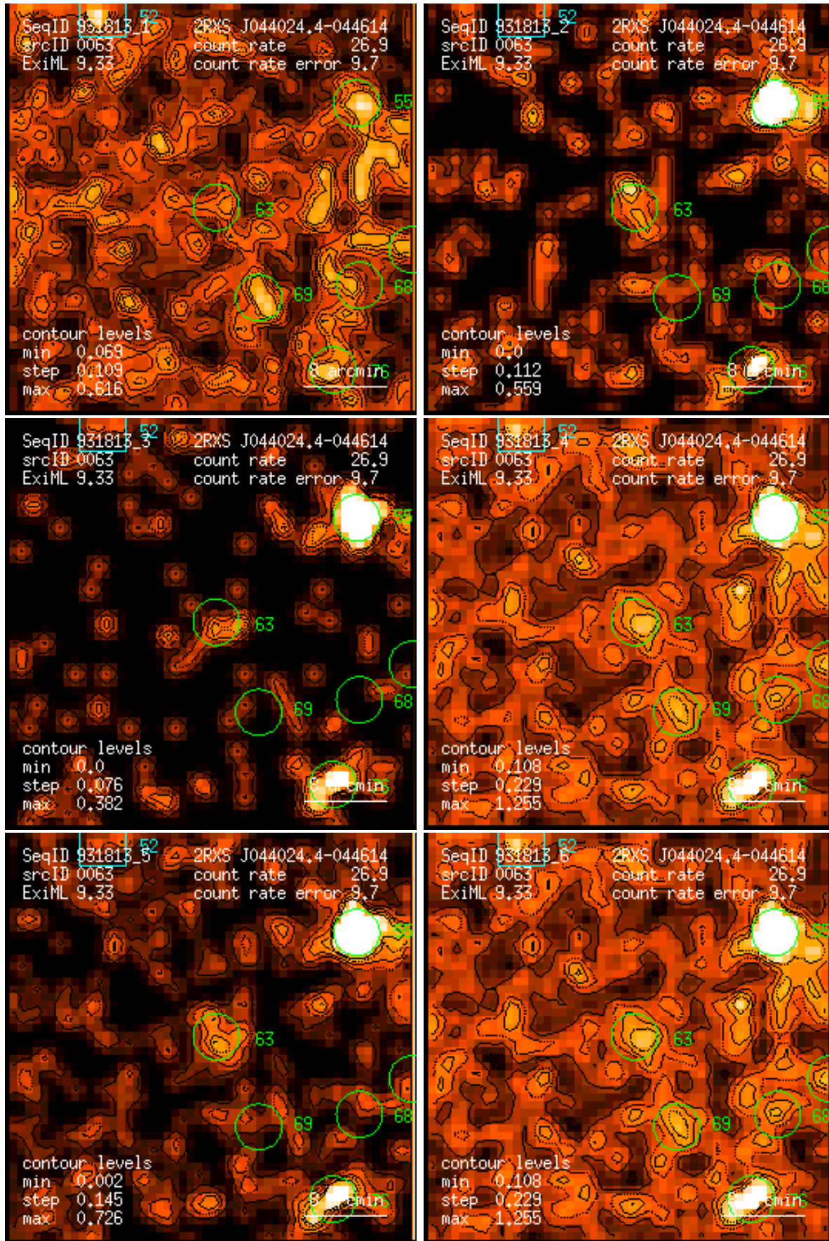
Figure 63: RASS 931813: detection 0063: band rate images, Gaussian filter: (1) PSPC channels 11 – 41, (2) 52 – 90, (3) 91 – 201, (4) 11 – 235, (5) 52 – 201, (6) 11 – 201. Broad band rates in counts/ks. Band rate contour levels in counts/ks/arcmin 2 .
