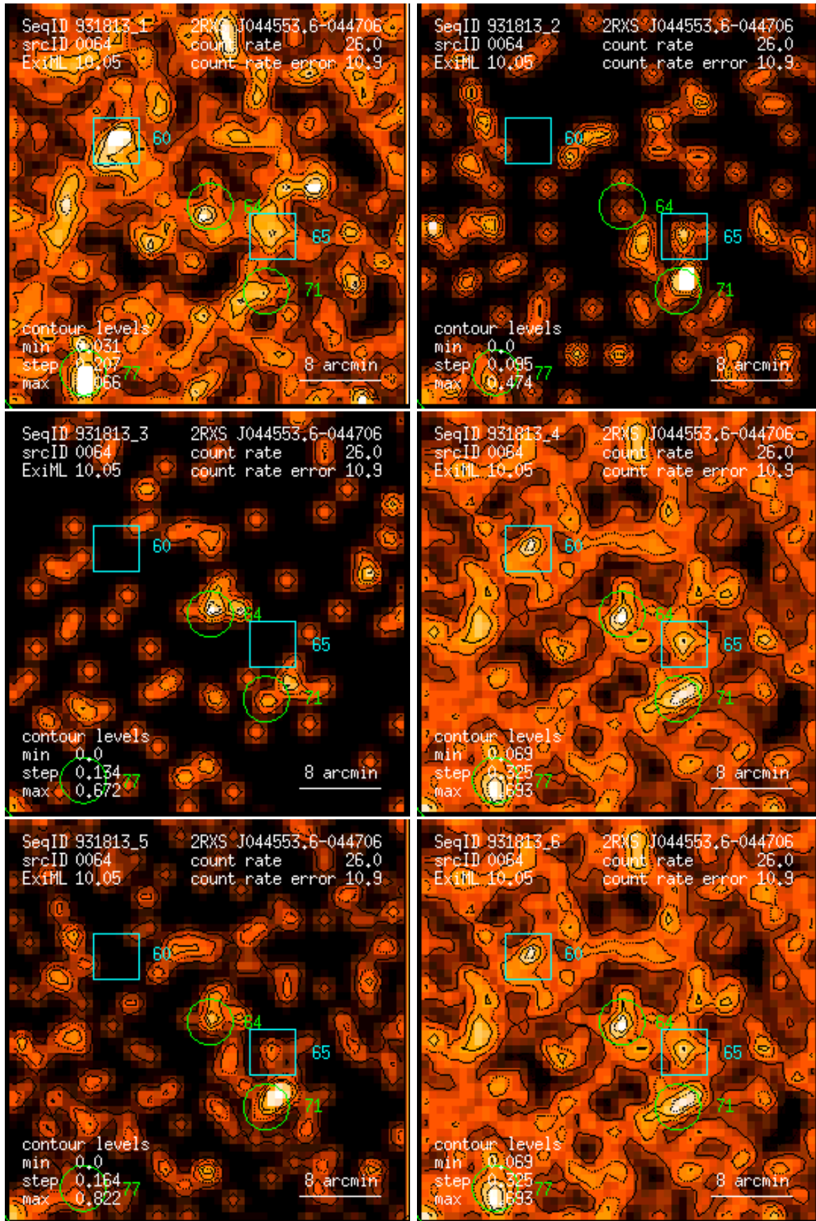
Figure 64: RASS 931813: detection 0064: band rate images, Gaussian filter: (1) PSPC channels 11 – 41, (2) 52 – 90, (3) 91 – 201, (4) 11 – 235, (5) 52 – 201, (6) 11 – 201. Broad band rates in counts/ks. Band rate contour levels in counts/ks/arcmin 2 .
