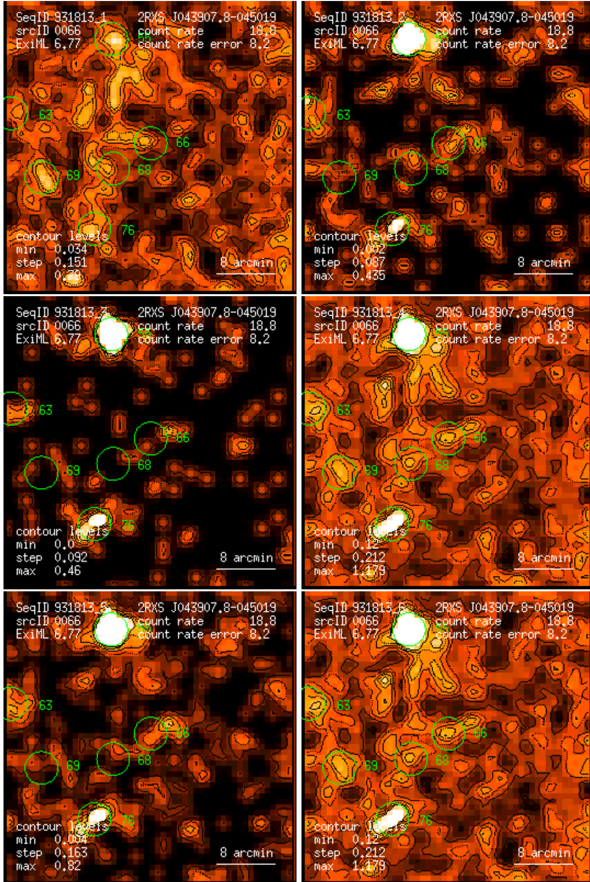
Figure 66: RASS 931813: detection 0066: band rate images, Gaussian filter: (1) PSPC channels 11 – 41, (2) 52 – 90, (3) 91 – 201, (4) 11 – 235, (5) 52 – 201, (6) 11 – 201. Broad band rates in counts/ks. Band rate contour levels in counts/ks/arcmin 2 .
