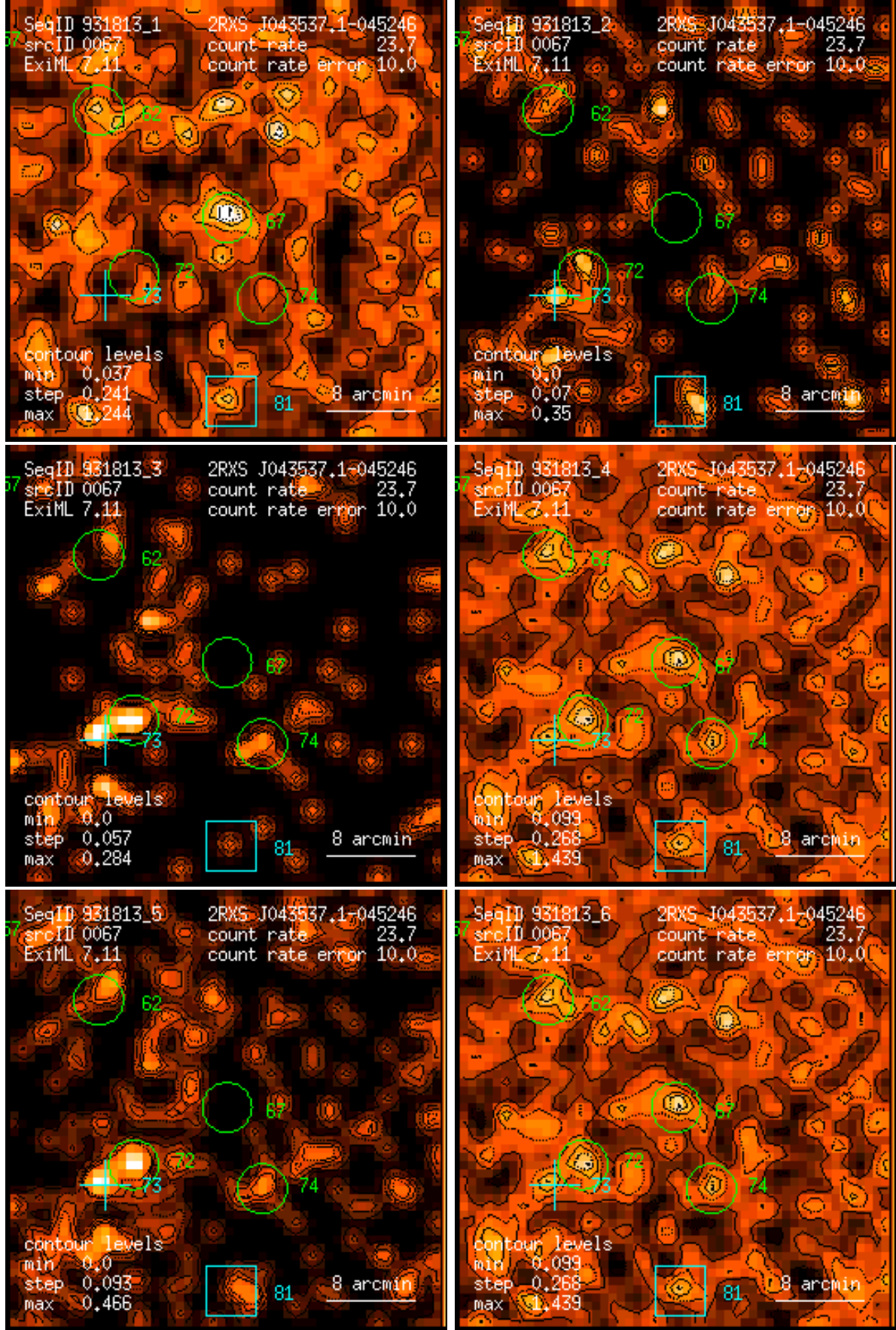
Figure 67: RASS 931813: detection 0067: band rate images, Gaussian filter: (1) PSPC channels 11 – 41, (2) 52 – 90, (3) 91 – 201, (4) 11 – 235, (5) 52 – 201, (6) 11 – 201. Broad band rates in counts/ks. Band rate contour levels in counts/ks/arcmin 2 .
