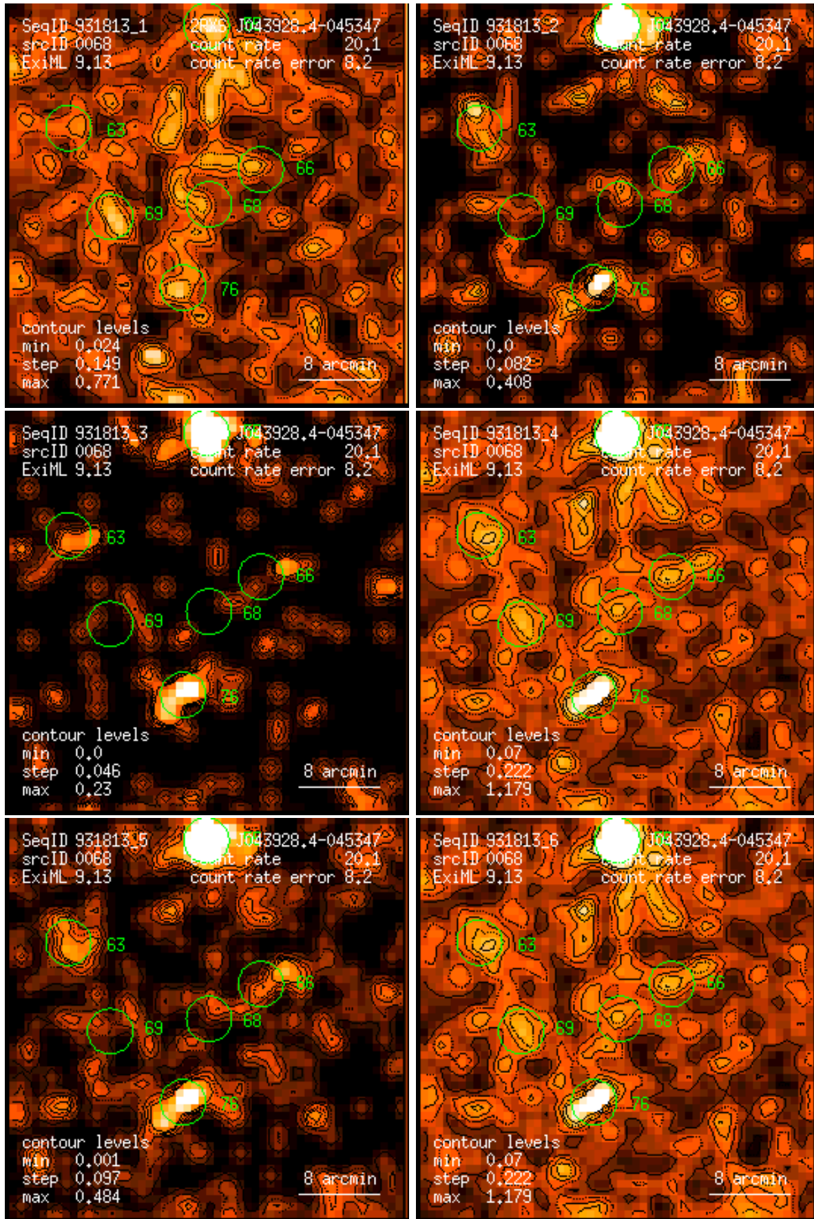
Figure 68: RASS 931813: detection 0068: band rate images, Gaussian filter: (1) PSPC channels 11 – 41, (2) 52 – 90, (3) 91 – 201, (4) 11 – 235, (5) 52 – 201, (6) 11 – 201. Broad band rates in counts/ks. Band rate contour levels in counts/ks/arcmin 2 .
