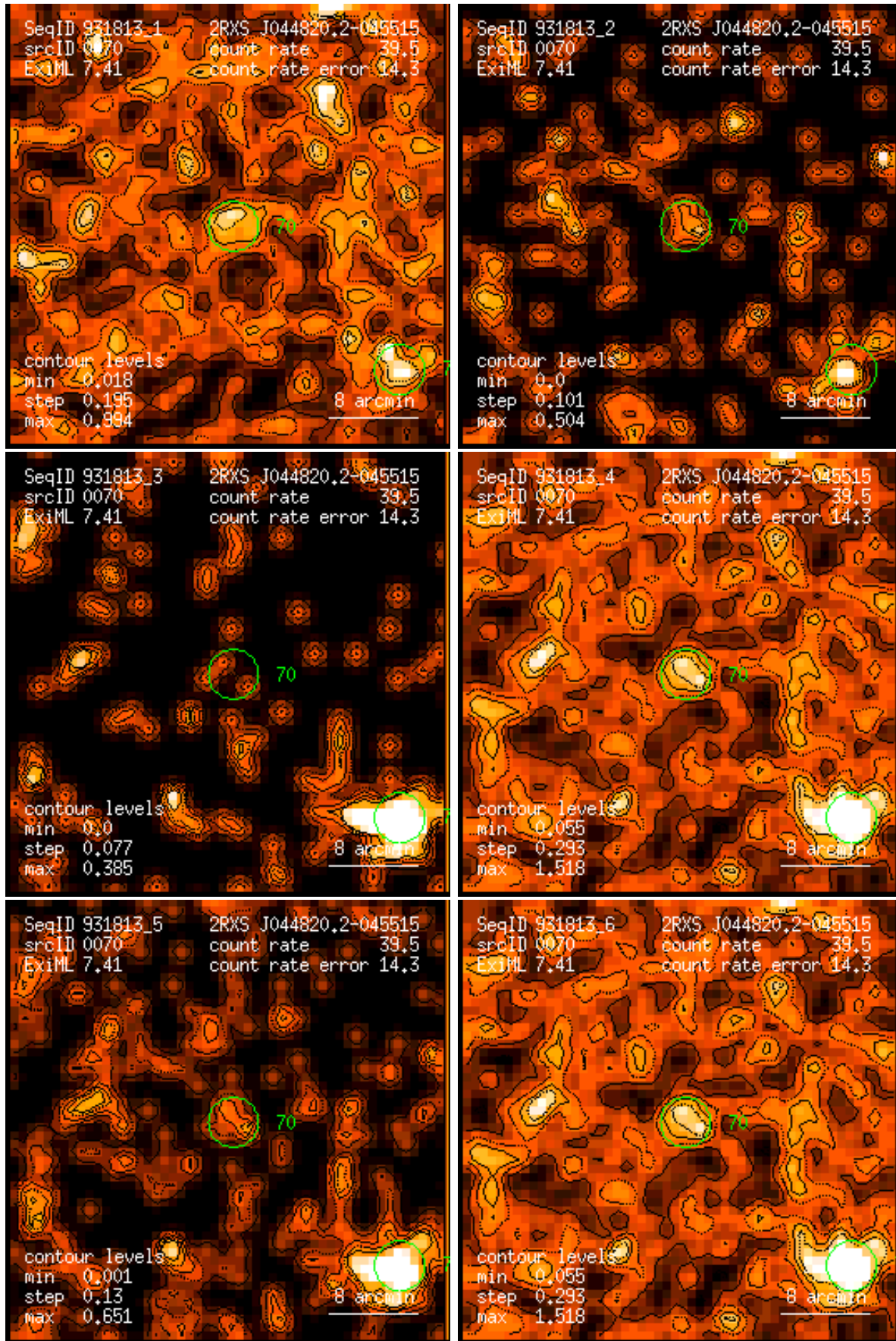
Figure 70: RASS 931813: detection 0070: band rate images, Gaussian filter: (1) PSPC channels 11 – 41, (2) 52 – 90, (3) 91 – 201, (4) 11 – 235, (5) 52 – 201, (6) 11 – 201. Broad band rates in counts/ks. Band rate contour levels in counts/ks/arcmin 2 .
