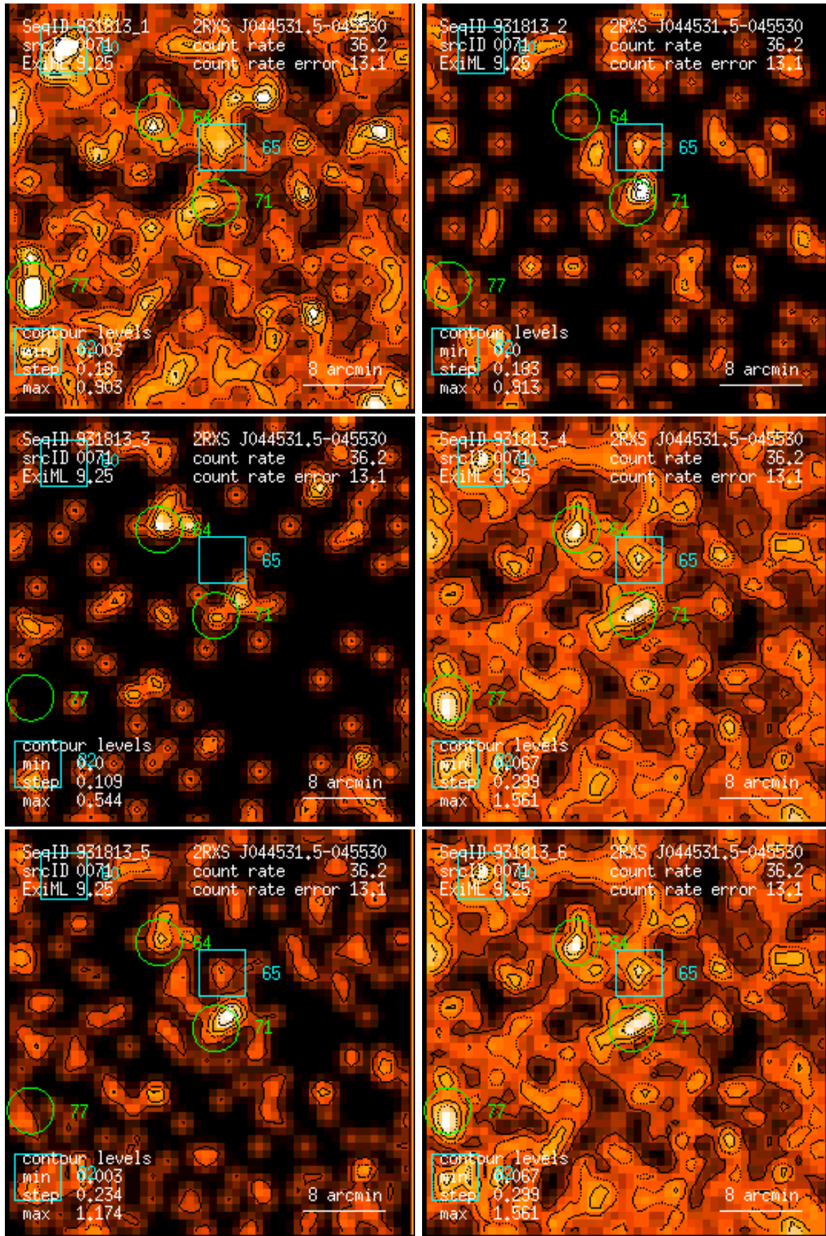
Figure 71: RASS 931813: detection 0071: band rate images, Gaussian filter: (1) PSPC channels 11 – 41, (2) 52 – 90, (3) 91 – 201, (4) 11 – 235, (5) 52 – 201, (6) 11 – 201. Broad band rates in counts/ks. Band rate contour levels in counts/ks/arcmin 2 .
