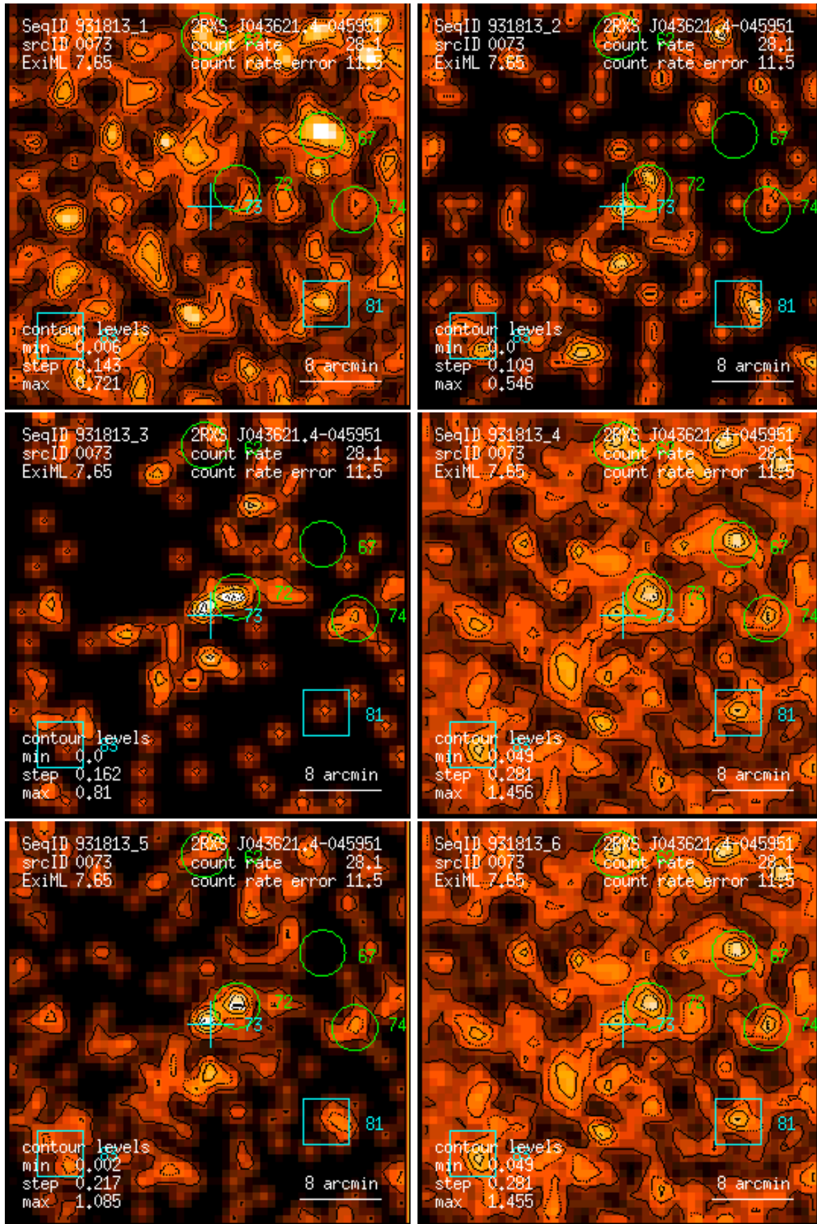
Figure 73: RASS 931813: detection 0073: band rate images, Gaussian filter: (1) PSPC channels 11 – 41, (2) 52 – 90, (3) 91 – 201, (4) 11 – 235, (5) 52 – 201, (6) 11 – 201. Broad band rates in counts/ks. Band rate contour levels in counts/ks/arcmin 2 .
