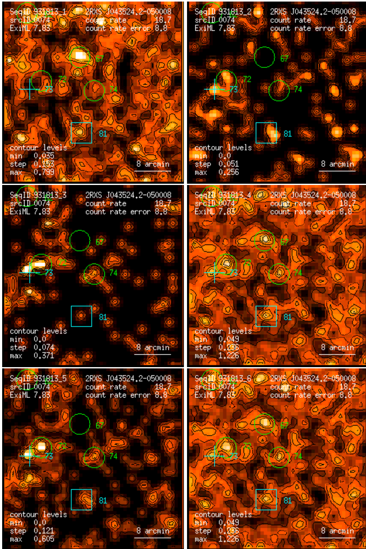
Figure 74: RASS 931813: detection 0074: band rate images, Gaussian filter: (1) PSPC channels 11 – 41, (2) 52 – 90, (3) 91 – 201, (4) 11 – 235, (5) 52 – 201, (6) 11 – 201. Broad band rates in counts/ks. Band rate contour levels in counts/ks/arcmin 2 .
