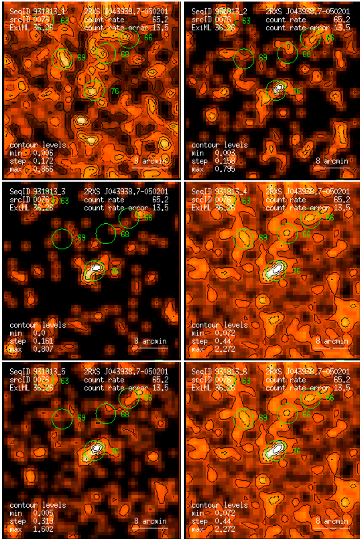
Figure 76: RASS 931813: detection 0076: band rate images, Gaussian filter: (1) PSPC channels 11 – 41, (2) 52 – 90, (3) 91 – 201, (4) 11 – 235, (5) 52 – 201, (6) 11 – 201. Broad band rates in counts/ks. Band rate contour levels in counts/ks/arcmin 2 .
