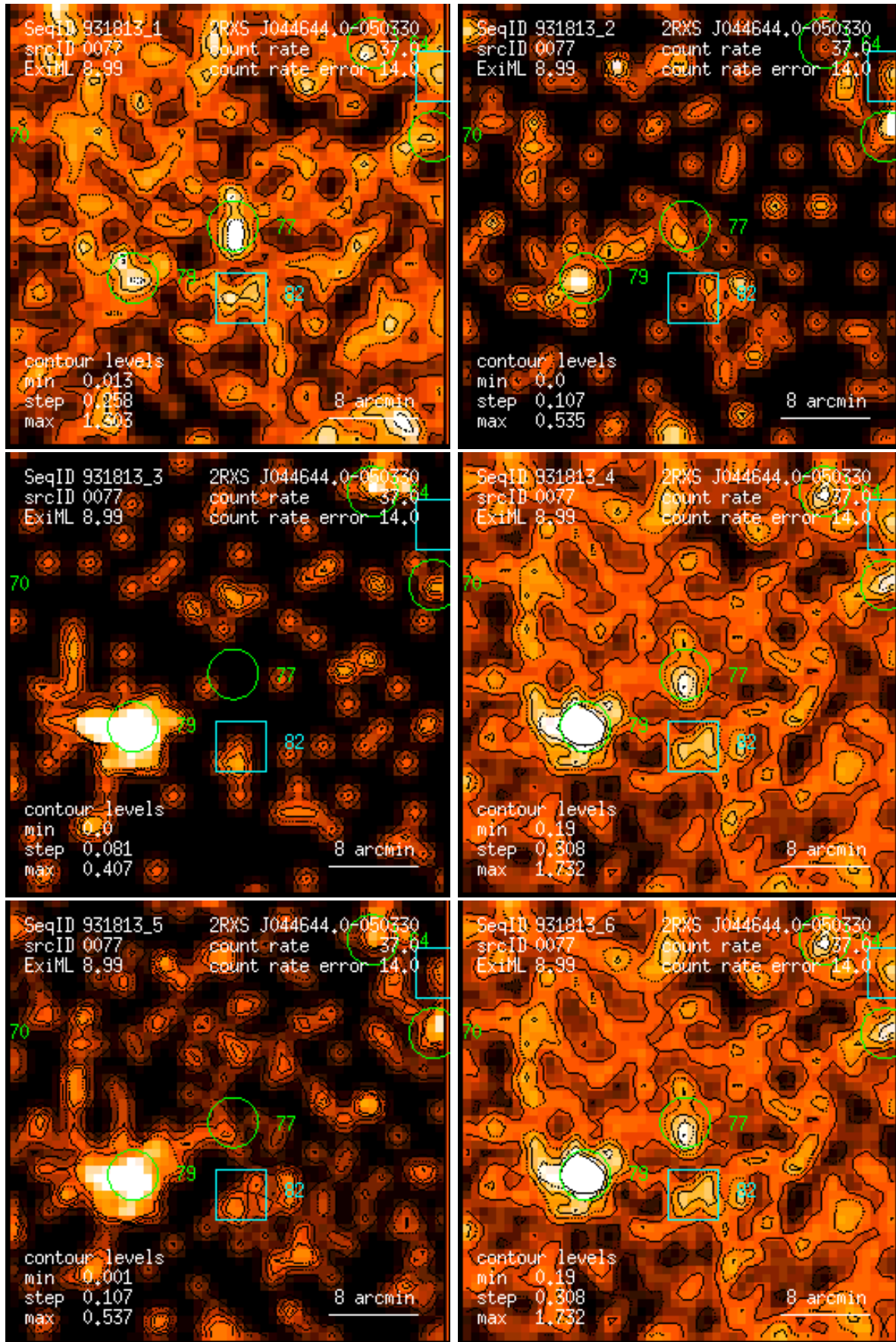
Figure 77: RASS 931813: detection 0077: band rate images, Gaussian filter: (1) PSPC channels 11 – 41, (2) 52 – 90, (3) 91 – 201, (4) 11 – 235, (5) 52 – 201, (6) 11 – 201. Broad band rates in counts/ks. Band rate contour levels in counts/ks/arcmin 2 .
