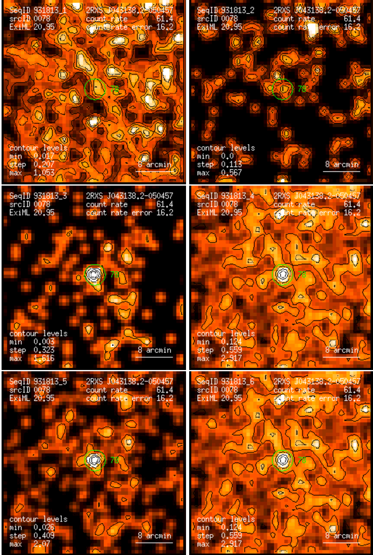
Figure 78: RASS 931813: detection 0078: band rate images, Gaussian filter: (1) PSPC channels 11 – 41, (2) 52 – 90, (3) 91 – 201, (4) 11 – 235, (5) 52 – 201, (6) 11 – 201. Broad band rates in counts/ks. Band rate contour levels in counts/ks/arcmin 2 .
