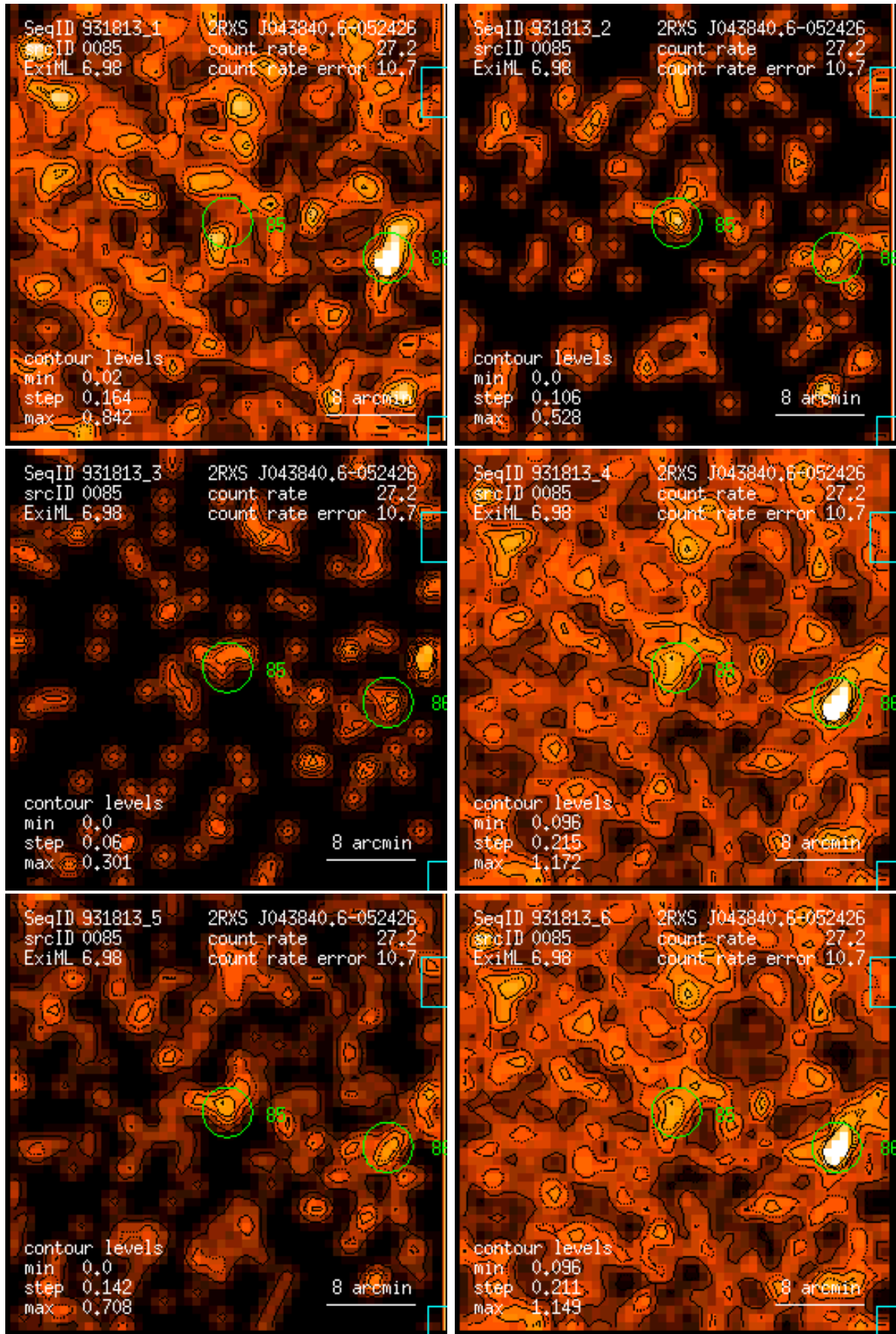
Figure 85: RASS 931813: detection 0085: band rate images, Gaussian filter: (1) PSPC channels 11 – 41, (2) 52 – 90, (3) 91 – 201, (4) 11 – 235, (5) 52 – 201, (6) 11 – 201. Broad band rates in counts/ks. Band rate contour levels in counts/ks/arcmin 2 .
