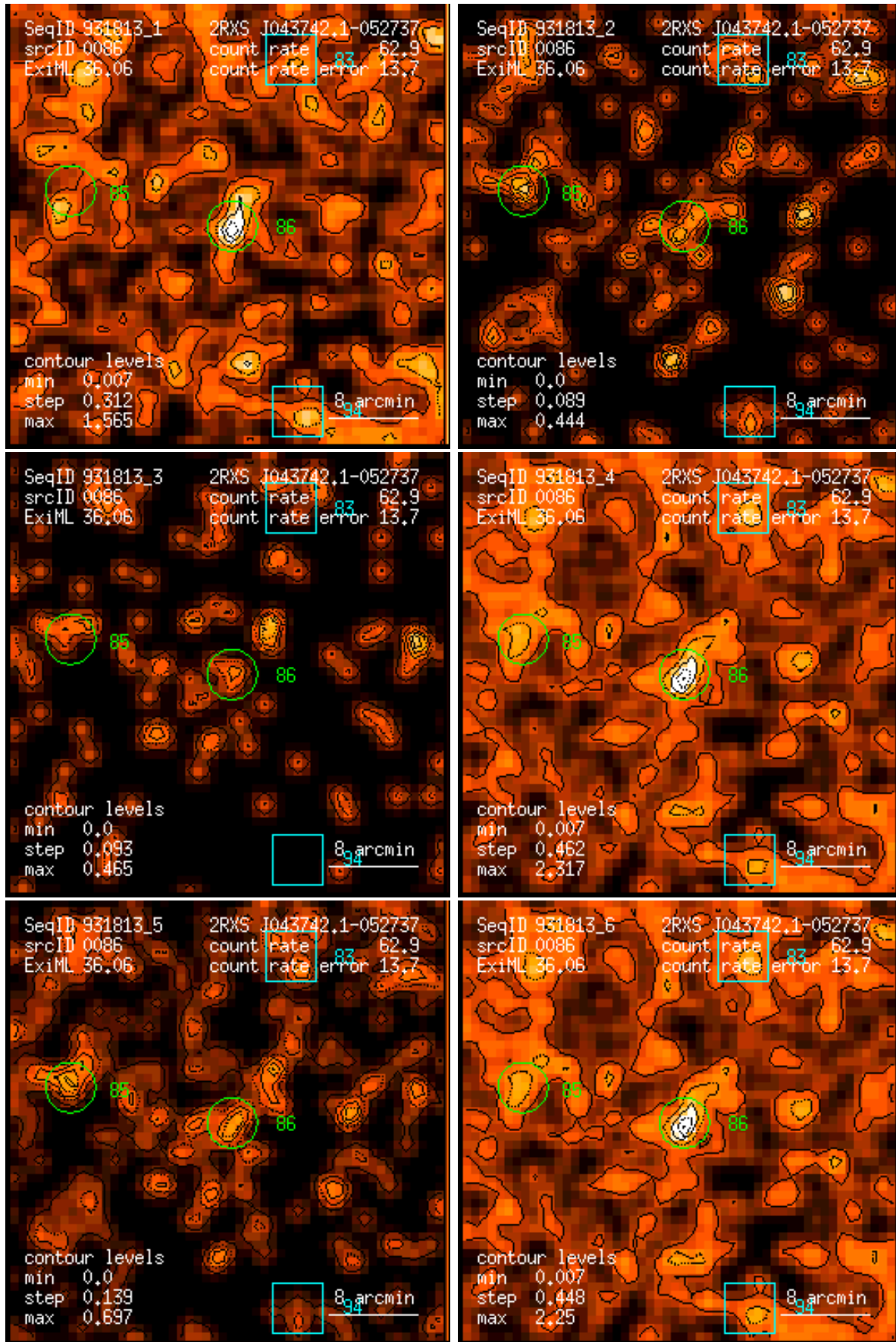
Figure 86: RASS 931813: detection 0086: band rate images, Gaussian filter: (1) PSPC channels 11 – 41, (2) 52 – 90, (3) 91 – 201, (4) 11 – 235, (5) 52 – 201, (6) 11 – 201. Broad band rates in counts/ks. Band rate contour levels in counts/ks/arcmin 2 .
