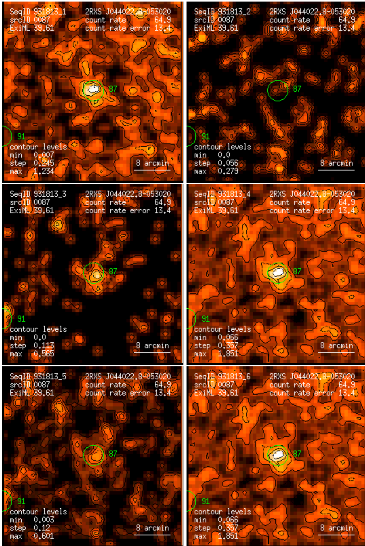
Figure 87: RASS 931813: detection 0087: band rate images, Gaussian filter: (1) PSPC channels 11 – 41, (2) 52 – 90, (3) 91 – 201, (4) 11 – 235, (5) 52 – 201, (6) 11 – 201. Broad band rates in counts/ks. Band rate contour levels in counts/ks/arcmin 2 .
