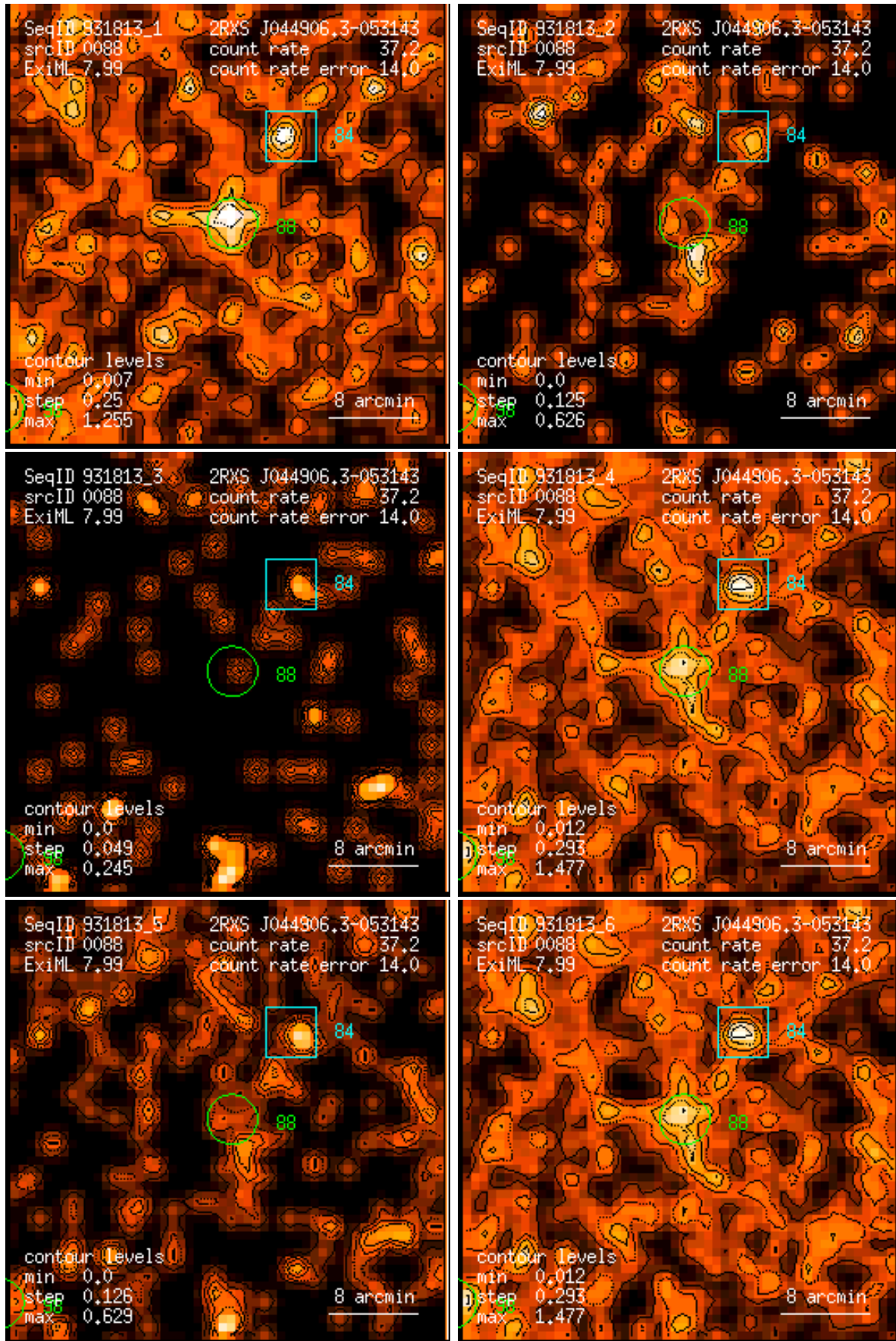
Figure 88: RASS 931813: detection 0088: band rate images, Gaussian filter: (1) PSPC channels 11 – 41, (2) 52 – 90, (3) 91 – 201, (4) 11 – 235, (5) 52 – 201, (6) 11 – 201. Broad band rates in counts/ks. Band rate contour levels in counts/ks/arcmin 2 .
