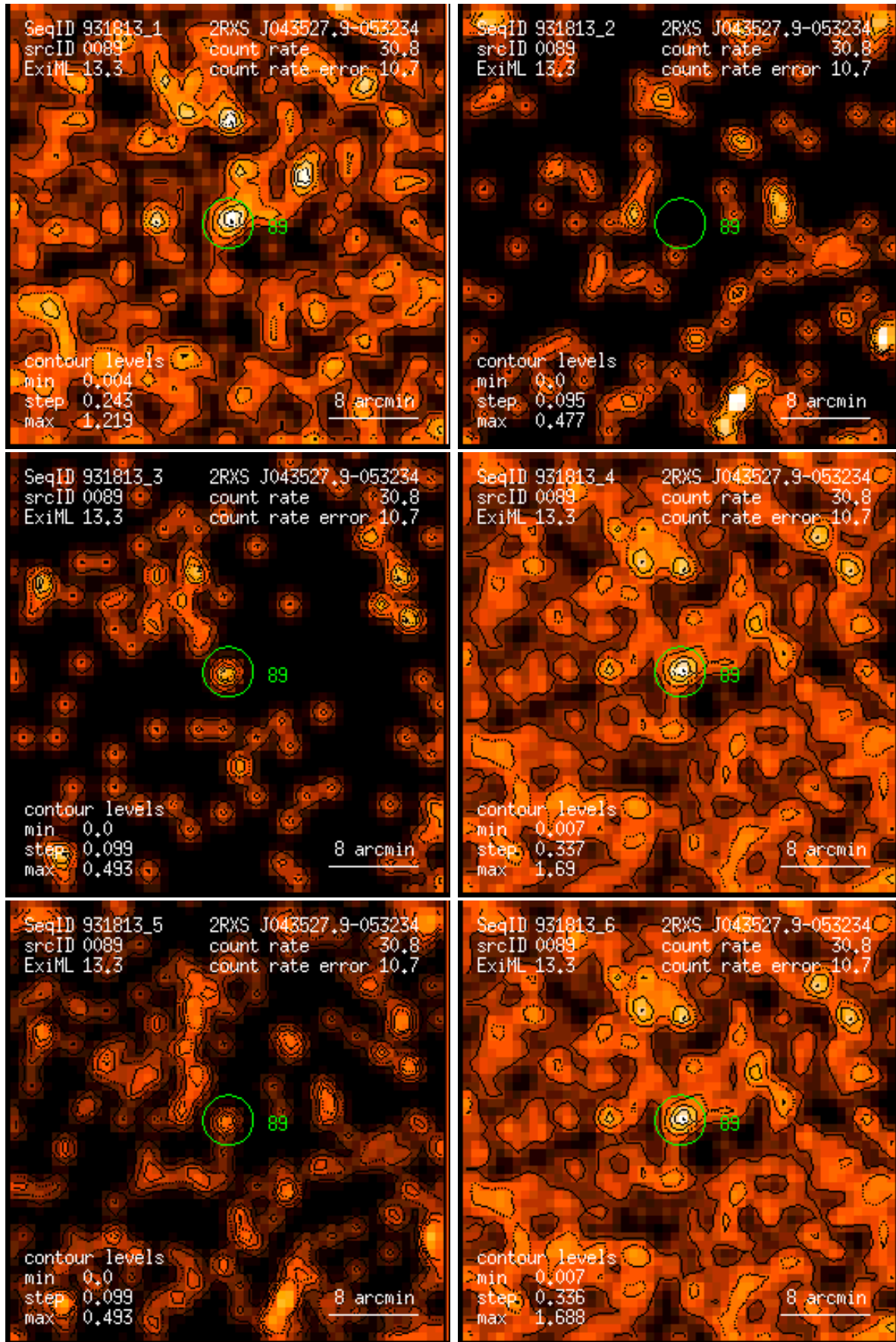
Figure 89: RASS 931813: detection 0089: band rate images, Gaussian filter: (1) PSPC channels 11 – 41, (2) 52 – 90, (3) 91 – 201, (4) 11 – 235, (5) 52 – 201, (6) 11 – 201. Broad band rates in counts/ks. Band rate contour levels in counts/ks/arcmin 2 .
