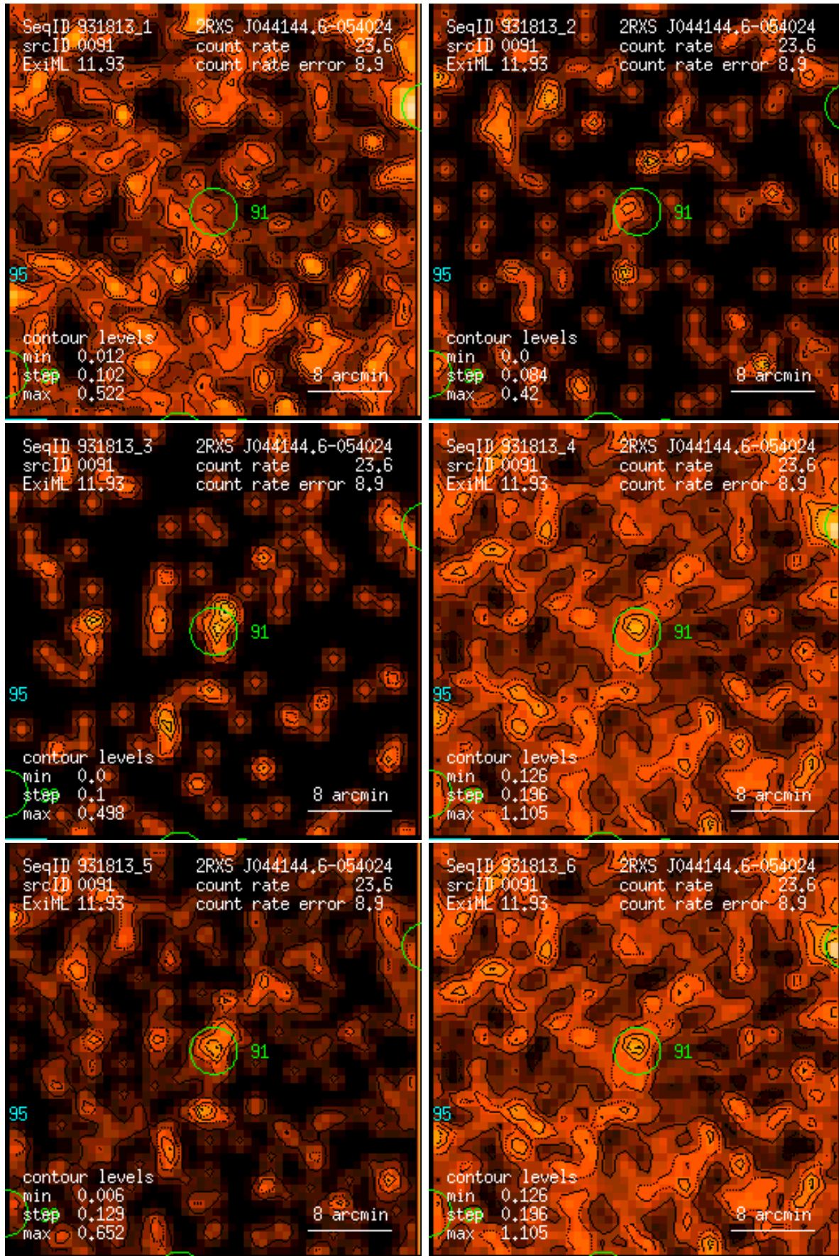
Figure 91: RASS 931813: detection 0091: band rate images, Gaussian filter: (1) PSPC channels 11 – 41, (2) 52 – 90, (3) 91 – 201, (4) 11 – 235, (5) 52 – 201, (6) 11 – 201. Broad band rates in counts/ks. Band rate contour levels in counts/ks/arcmin 2 .
