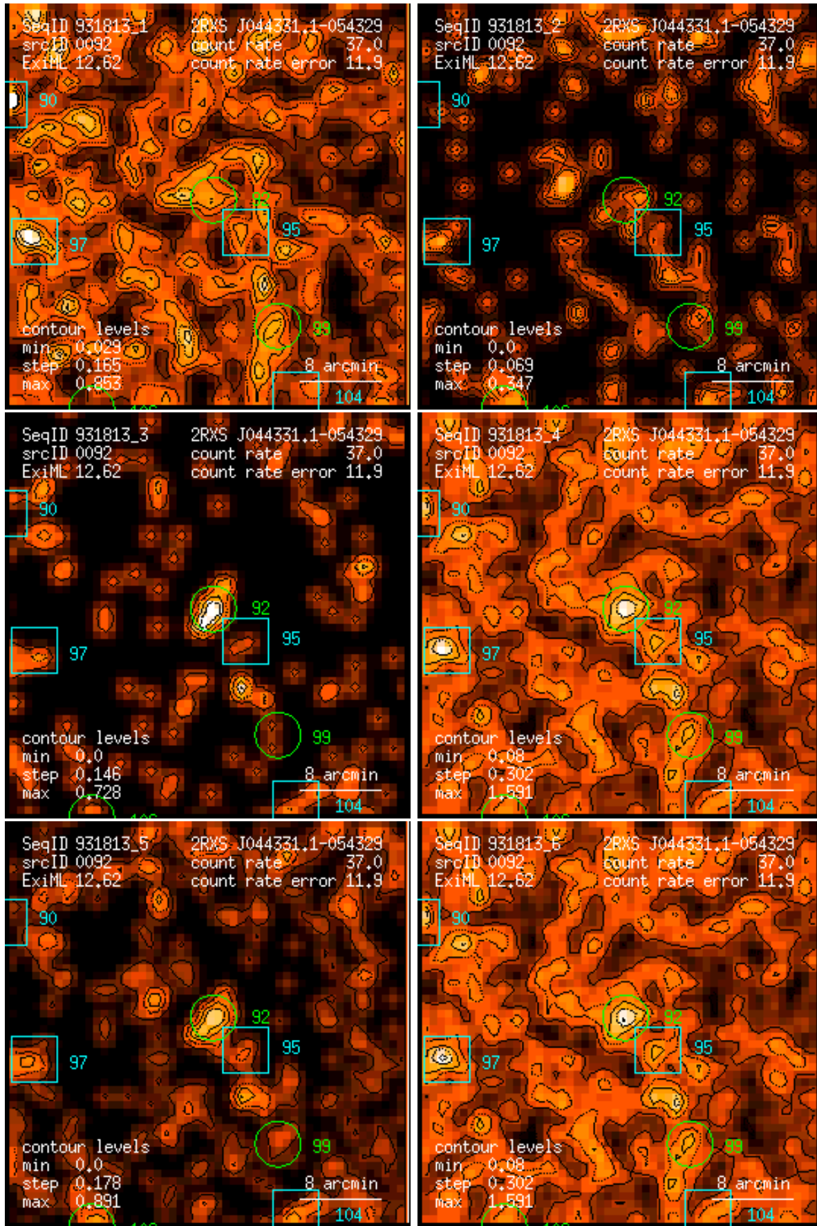
Figure 92: RASS 931813: detection 0092: band rate images, Gaussian filter: (1) PSPC channels 11 – 41, (2) 52 – 90, (3) 91 – 201, (4) 11 – 235, (5) 52 – 201, (6) 11 – 201. Broad band rates in counts/ks. Band rate contour levels in counts/ks/arcmin 2 .
