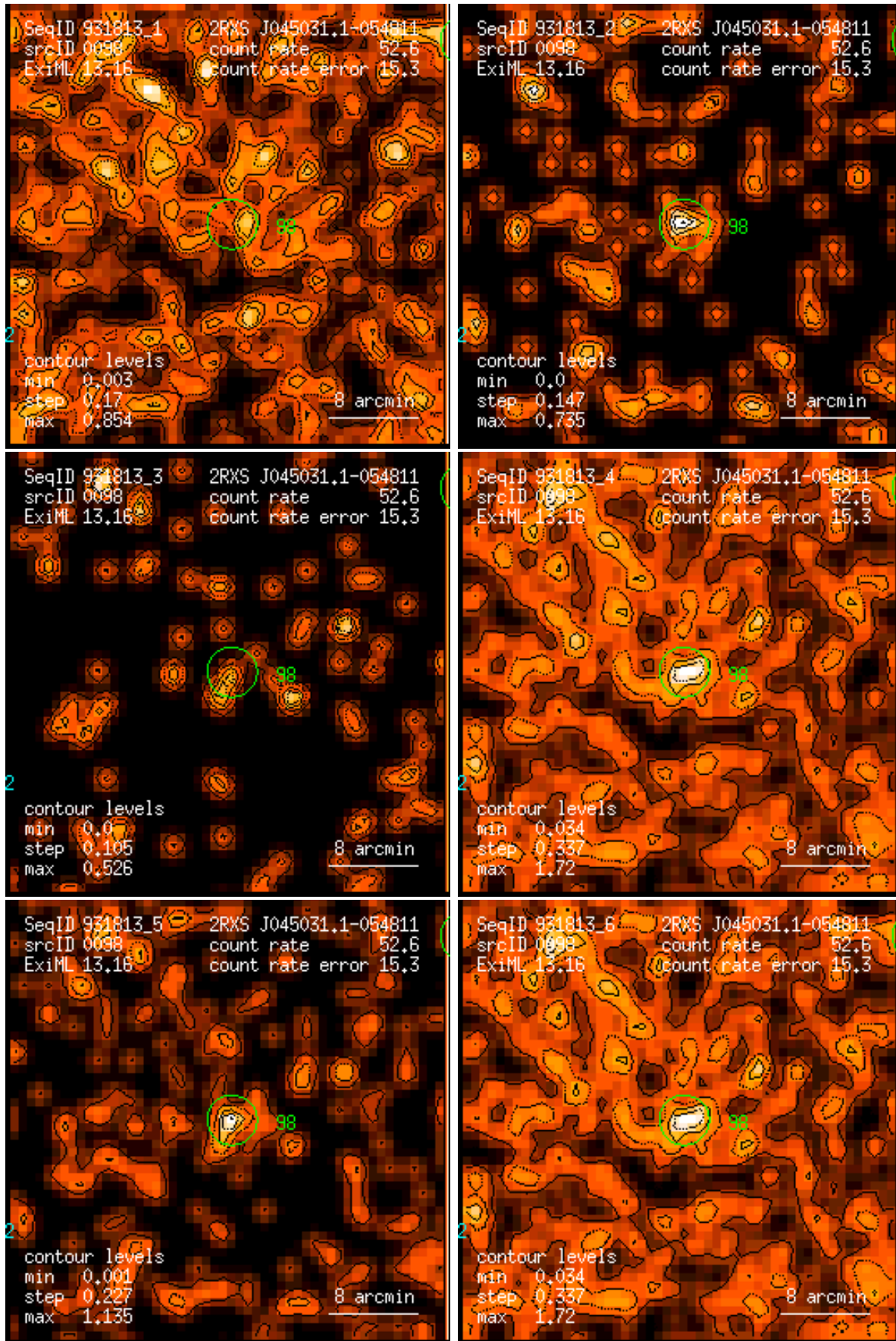
Figure 98: RASS 931813: detection 0098: band rate images, Gaussian filter: (1) PSPC channels 11 – 41, (2) 52 – 90, (3) 91 – 201, (4) 11 – 235, (5) 52 – 201, (6) 11 – 201. Broad band rates in counts/ks. Band rate contour levels in counts/ks/arcmin 2 .
