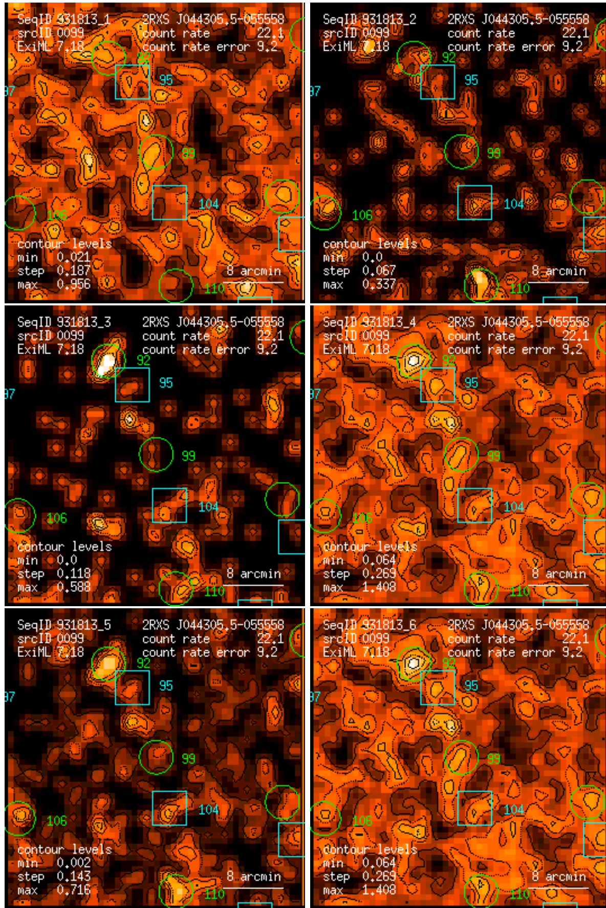
Figure 99: RASS 931813: detection 0099: band rate images, Gaussian filter: (1) PSPC channels 11 – 41, (2) 52 – 90, (3) 91 – 201, (4) 11 – 235, (5) 52 – 201, (6) 11 – 201. Broad band rates in counts/ks. Band rate contour levels in counts/ks/arcmin 2 .
