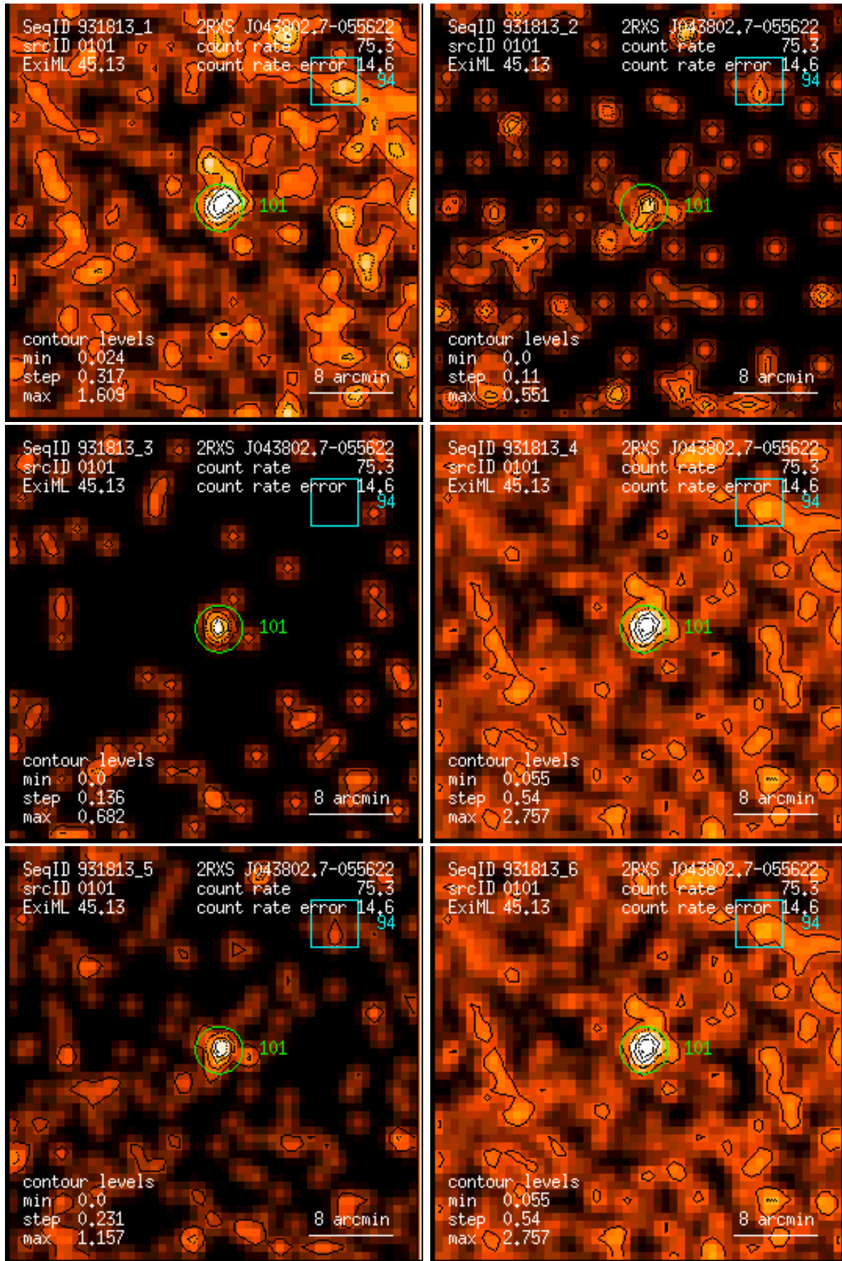
Figure 101: RASS 931813: detection 0101: band rate images, Gaussian filter: (1) PSPC channels 11 – 41, (2) 52 – 90, (3) 91 – 201, (4) 11 – 235, (5) 52 – 201, (6) 11 – 201. Broad band rates in counts/ks. Band rate contour levels in counts/ks/arcmin 2 .
