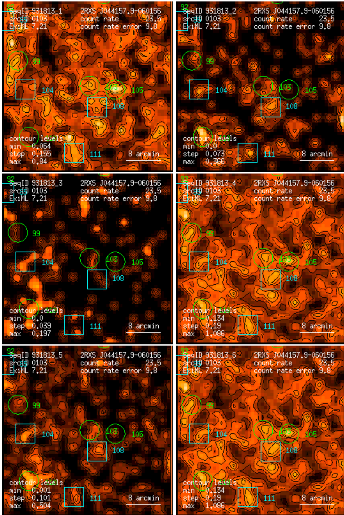
Figure 103: RASS 931813: detection 0103: band rate images, Gaussian filter: (1) PSPC channels 11 – 41, (2) 52 – 90, (3) 91 – 201, (4) 11 – 235, (5) 52 – 201, (6) 11 – 201. Broad band rates in counts/ks. Band rate contour levels in counts/ks/arcmin 2 .
