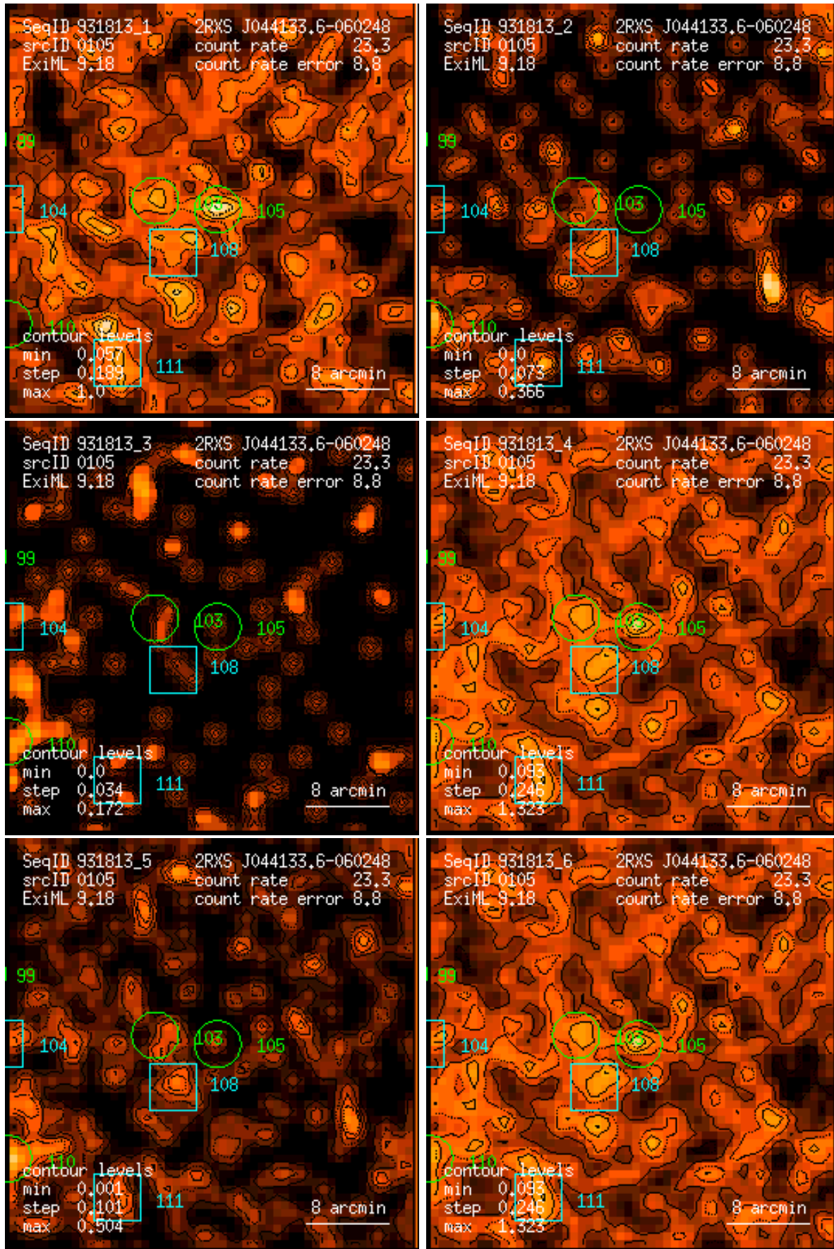
Figure 105: RASS 931813: detection 0105: band rate images, Gaussian filter: (1) PSPC channels 11 – 41, (2) 52 – 90, (3) 91 – 201, (4) 11 – 235, (5) 52 – 201, (6) 11 – 201. Broad band rates in counts/ks. Band rate contour levels in counts/ks/arcmin 2 .
