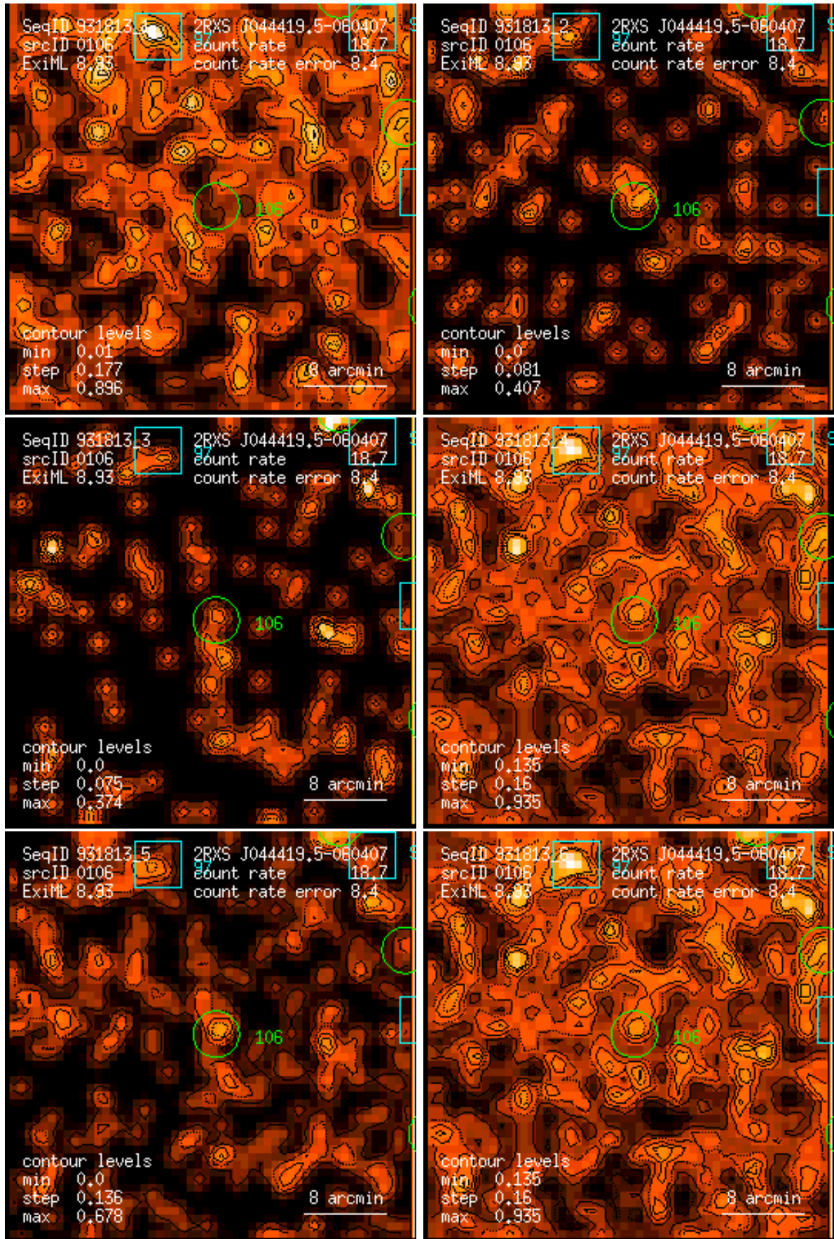
Figure 106: RASS 931813: detection 0106: band rate images, Gaussian filter: (1) PSPC channels 11 – 41, (2) 52 – 90, (3) 91 – 201, (4) 11 – 235, (5) 52 – 201, (6) 11 – 201. Broad band rates in counts/ks. Band rate contour levels in counts/ks/arcmin 2 .
