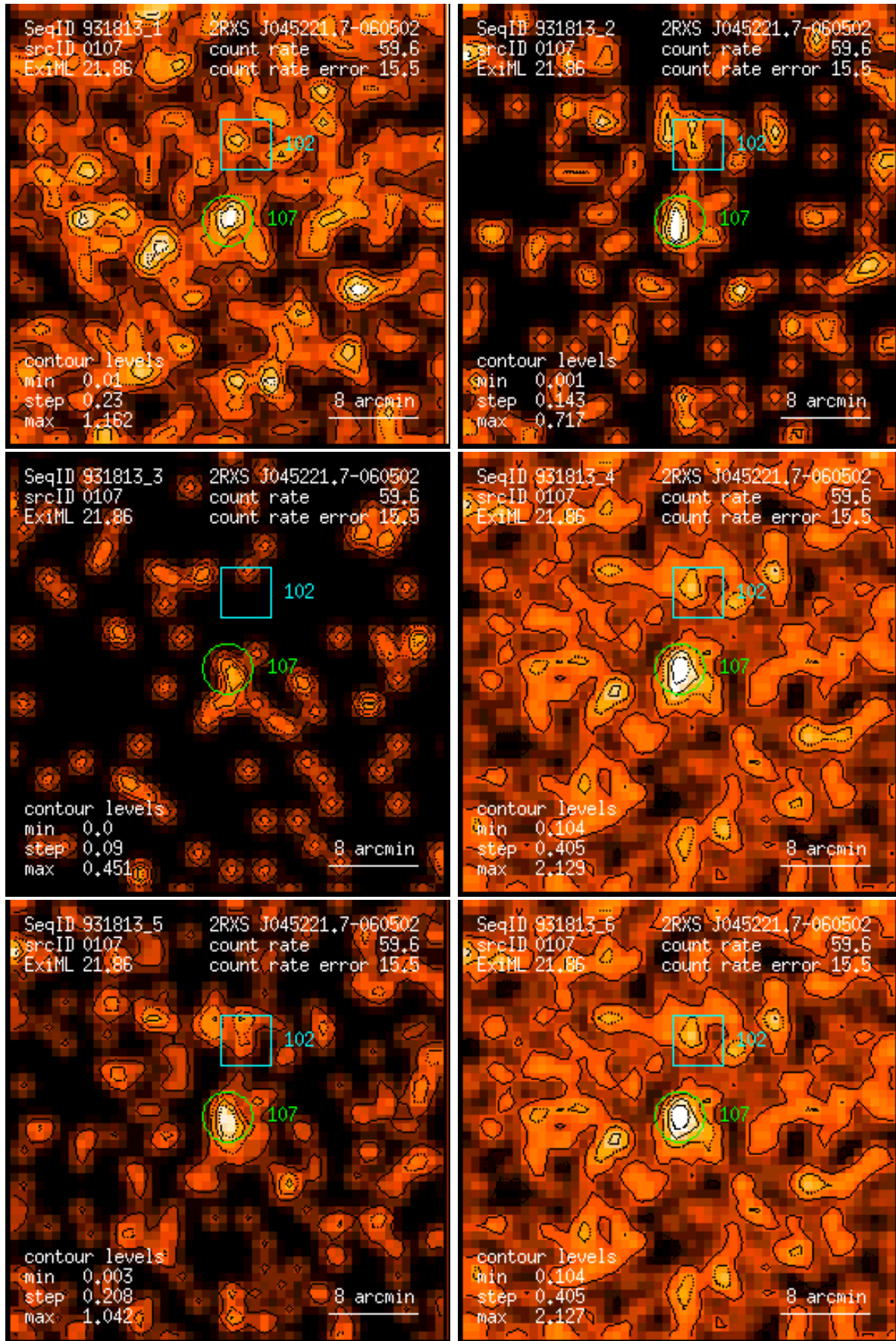
Figure 107: RASS 931813: detection 0107: band rate images, Gaussian filter: (1) PSPC channels 11 – 41, (2) 52 – 90, (3) 91 – 201, (4) 11 – 235, (5) 52 – 201, (6) 11 – 201. Broad band rates in counts/ks. Band rate contour levels in counts/ks/arcmin 2 .
