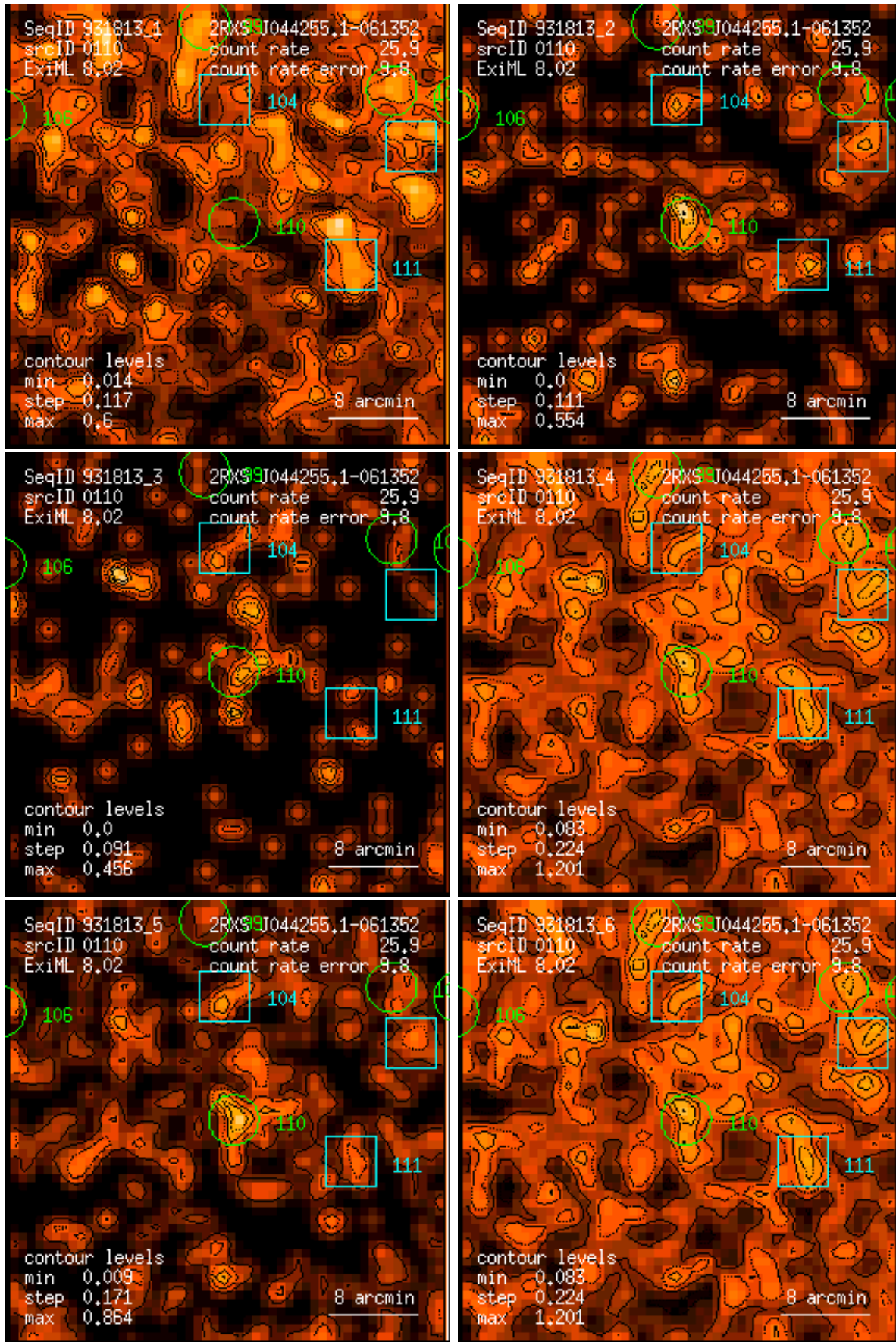
Figure 110: RASS 931813: detection 0110: band rate images, Gaussian filter: (1) PSPC channels 11 – 41, (2) 52 – 90, (3) 91 – 201, (4) 11 – 235, (5) 52 – 201, (6) 11 – 201. Broad band rates in counts/ks. Band rate contour levels in counts/ks/arcmin 2 .
