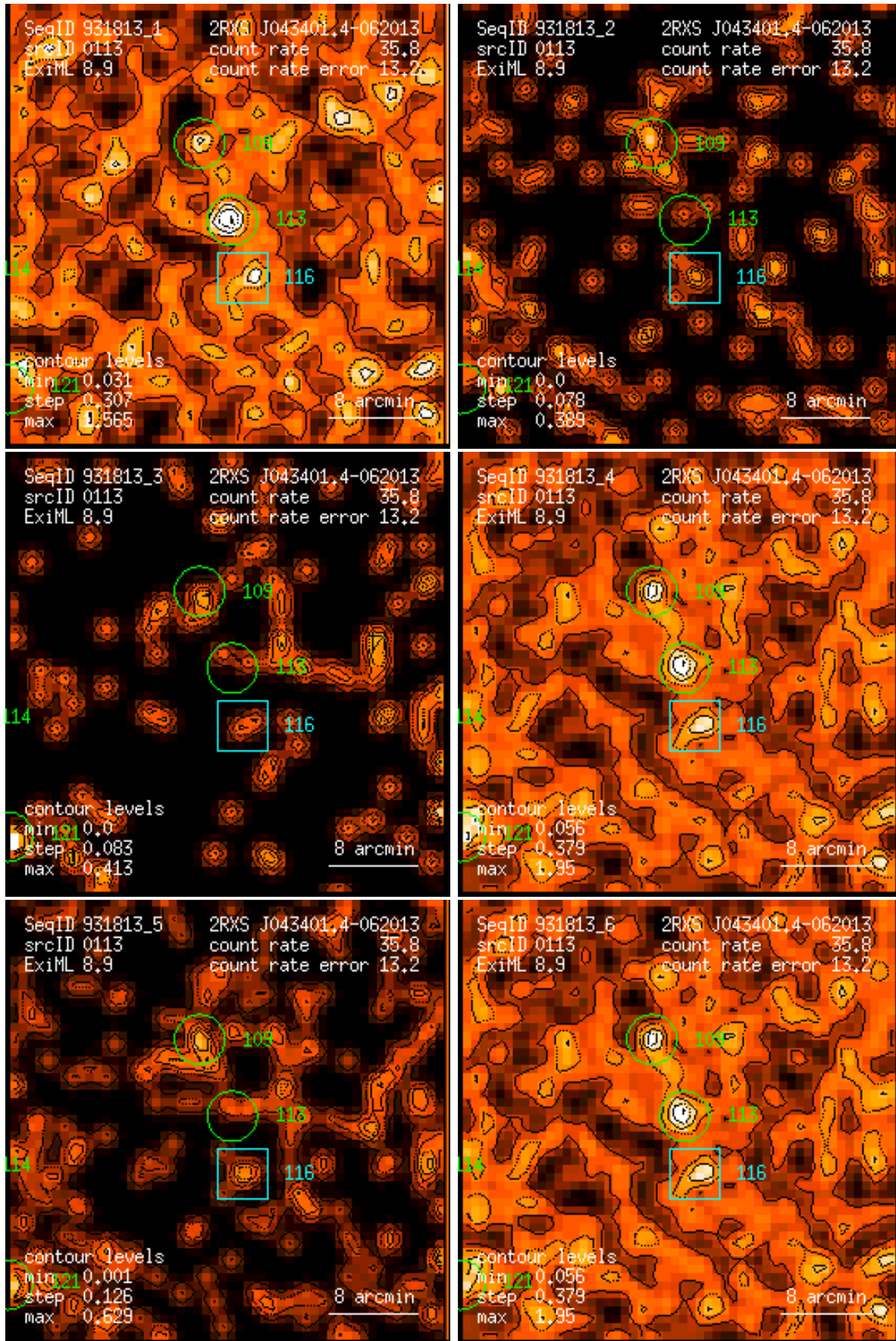
Figure 113: RASS 931813: detection 0113: band rate images, Gaussian filter: (1) PSPC channels 11 – 41, (2) 52 – 90, (3) 91 – 201, (4) 11 – 235, (5) 52 – 201, (6) 11 – 201. Broad band rates in counts/ks. Band rate contour levels in counts/ks/arcmin 2 .
