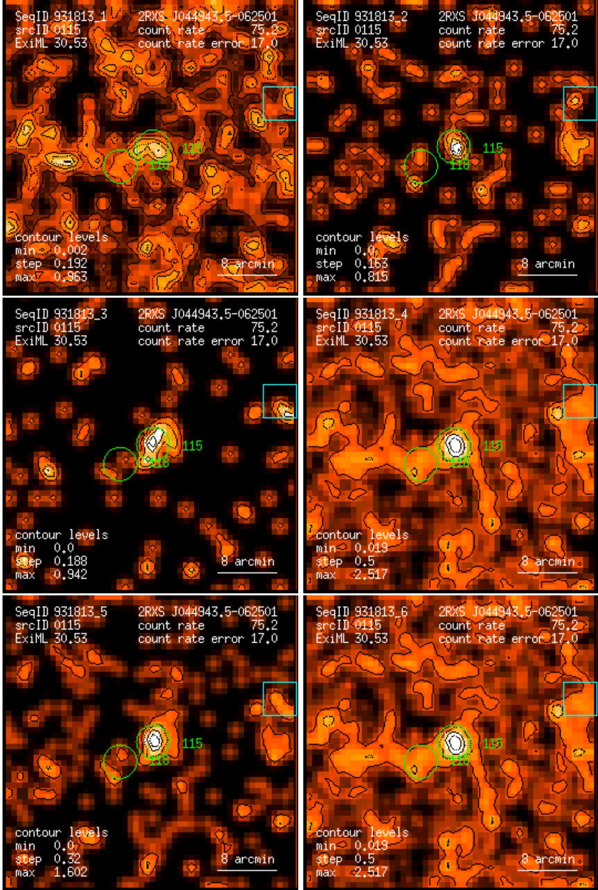
Figure 115: RASS 931813: detection 0115: band rate images, Gaussian filter: (1) PSPC channels 11 – 41, (2) 52 – 90, (3) 91 – 201, (4) 11 – 235, (5) 52 – 201, (6) 11 – 201. Broad band rates in counts/ks. Band rate contour levels in counts/ks/arcmin 2 .
