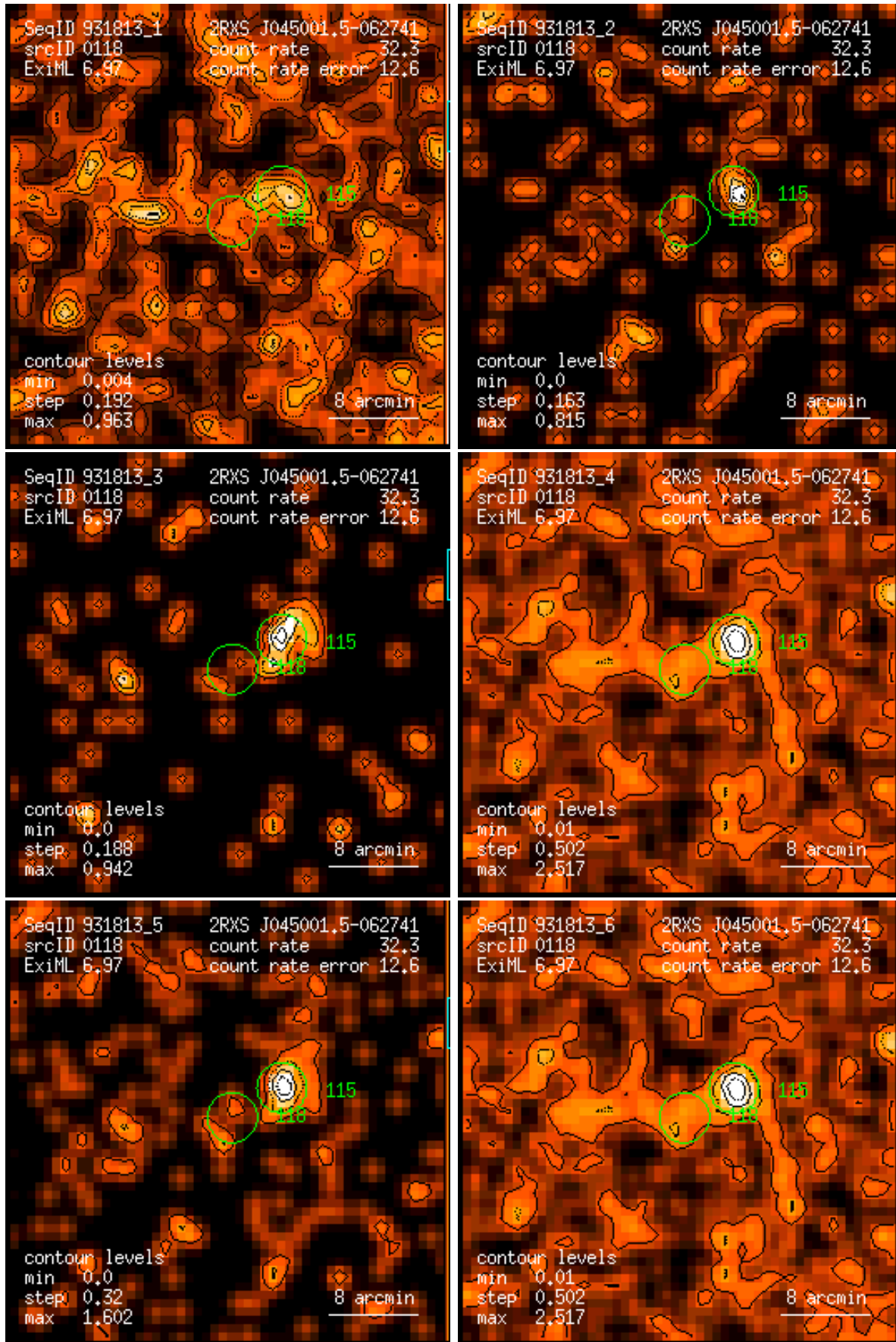
Figure 118: RASS 931813: detection 0118: band rate images, Gaussian filter: (1) PSPC channels 11 – 41, (2) 52 – 90, (3) 91 – 201, (4) 11 – 235, (5) 52 – 201, (6) 11 – 201. Broad band rates in counts/ks. Band rate contour levels in counts/ks/arcmin 2 .
