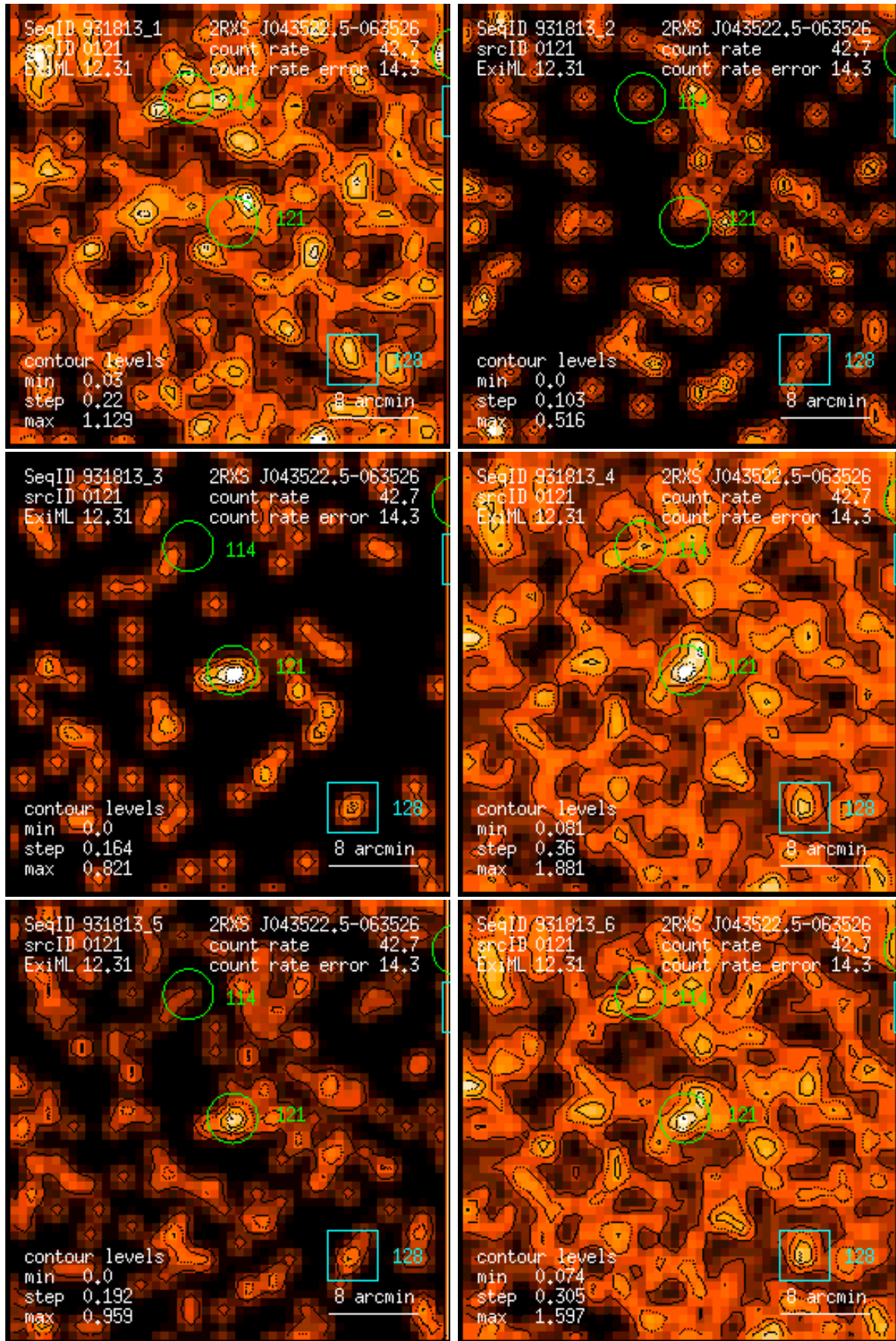
Figure 121: RASS 931813: detection 0121: band rate images, Gaussian filter: (1) PSPC channels 11 – 41, (2) 52 – 90, (3) 91 – 201, (4) 11 – 235, (5) 52 – 201, (6) 11 – 201. Broad band rates in counts/ks. Band rate contour levels in counts/ks/arcmin 2 .
