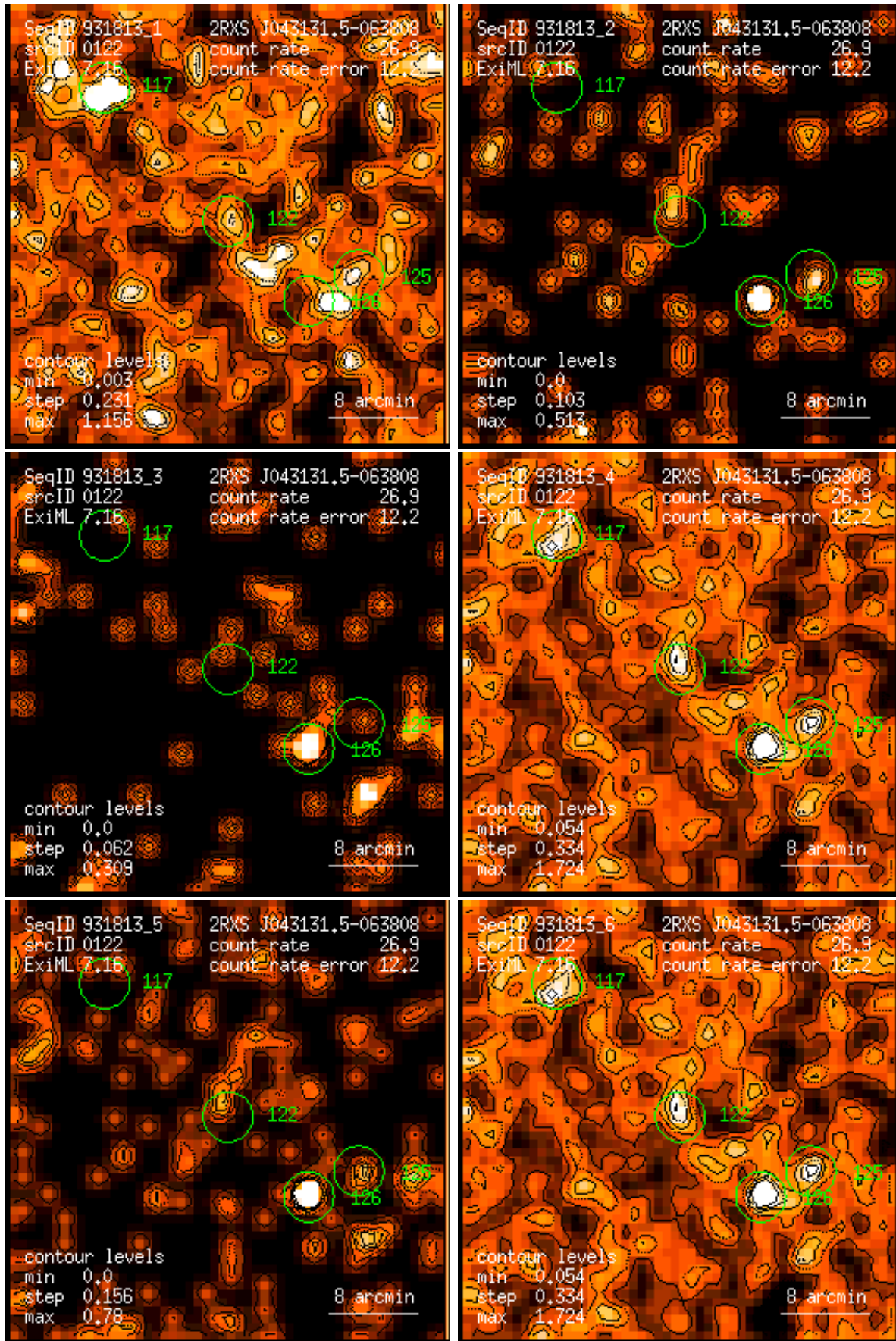
Figure 122: RASS 931813: detection 0122: band rate images, Gaussian filter: (1) PSPC channels 11 – 41, (2) 52 – 90, (3) 91 – 201, (4) 11 – 235, (5) 52 – 201, (6) 11 – 201. Broad band rates in counts/ks. Band rate contour levels in counts/ks/arcmin 2 .
