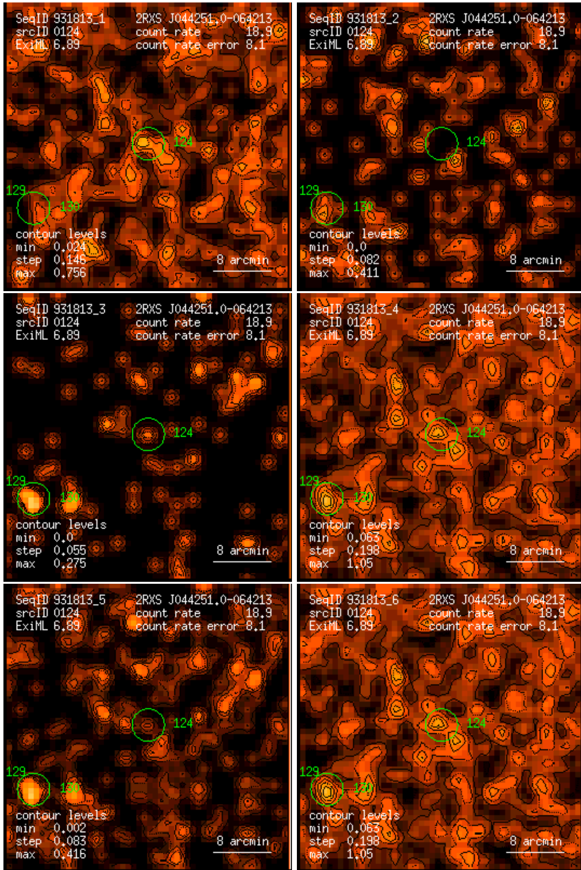
Figure 124: RASS 931813: detection 0124: band rate images, Gaussian filter: (1) PSPC channels 11 – 41, (2) 52 – 90, (3) 91 – 201, (4) 11 – 235, (5) 52 – 201, (6) 11 – 201. Broad band rates in counts/ks. Band rate contour levels in counts/ks/arcmin 2 .
