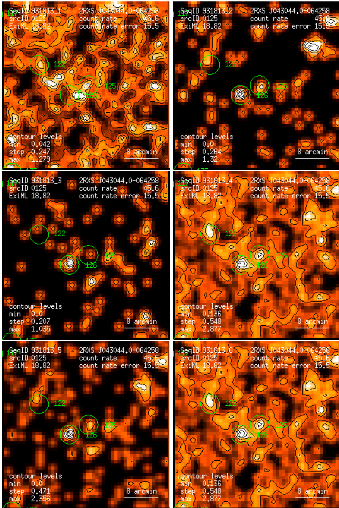
Figure 125: RASS 931813: detection 0125: band rate images, Gaussian filter: (1) PSPC channels 11 – 41, (2) 52 – 90, (3) 91 – 201, (4) 11 – 235, (5) 52 – 201, (6) 11 – 201. Broad band rates in counts/ks. Band rate contour levels in counts/ks/arcmin 2 .
