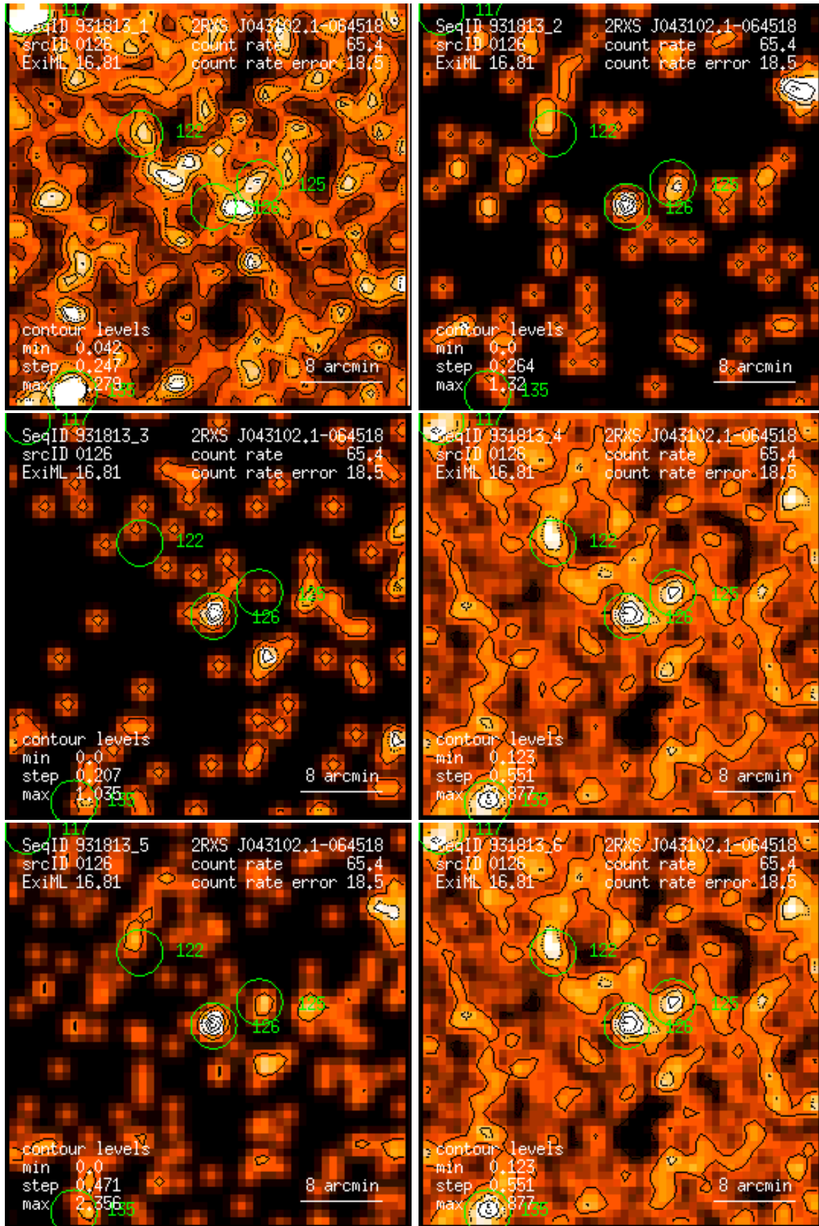
Figure 126: RASS 931813: detection 0126: band rate images, Gaussian filter: (1) PSPC channels 11 – 41, (2) 52 – 90, (3) 91 – 201, (4) 11 – 235, (5) 52 – 201, (6) 11 – 201. Broad band rates in counts/ks. Band rate contour levels in counts/ks/arcmin 2 .
