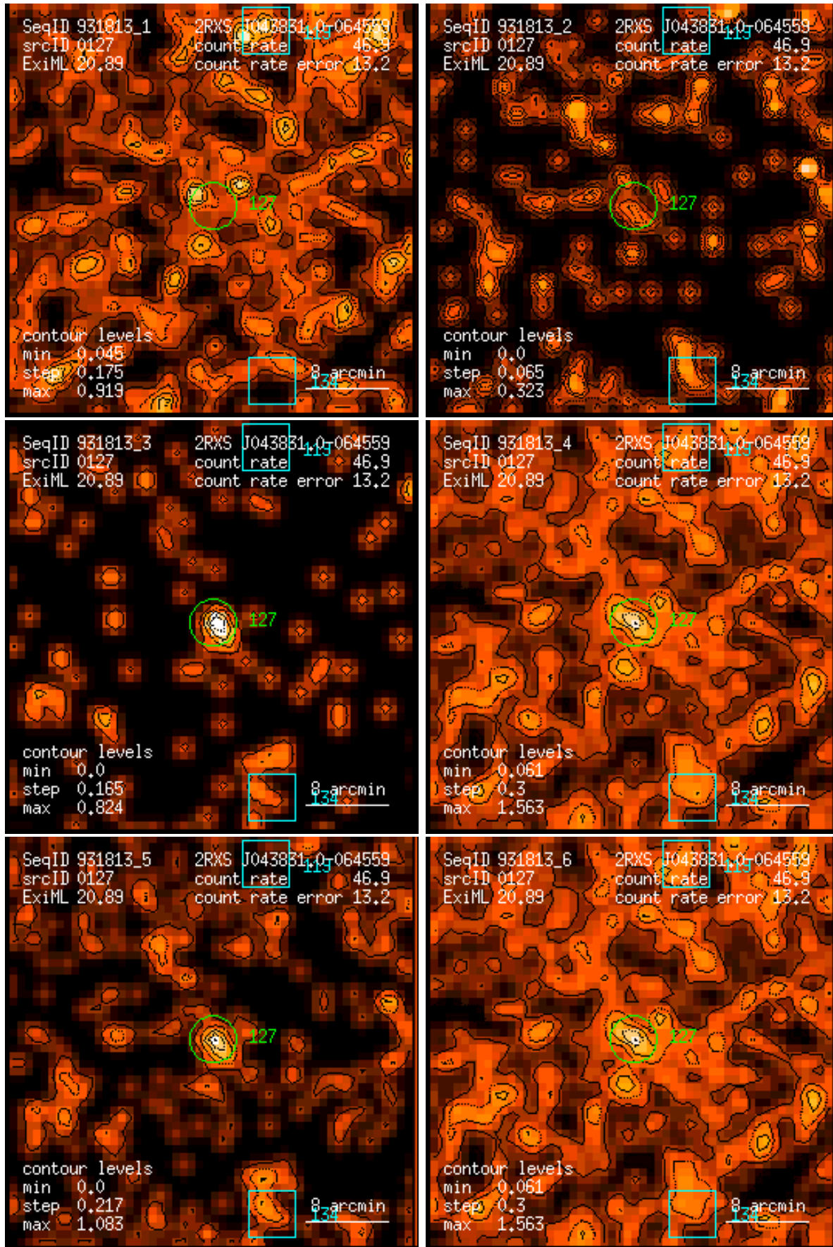
Figure 127: RASS 931813: detection 0127: band rate images, Gaussian filter: (1) PSPC channels 11 – 41, (2) 52 – 90, (3) 91 – 201, (4) 11 – 235, (5) 52 – 201, (6) 11 – 201. Broad band rates in counts/ks. Band rate contour levels in counts/ks/arcmin 2 .
