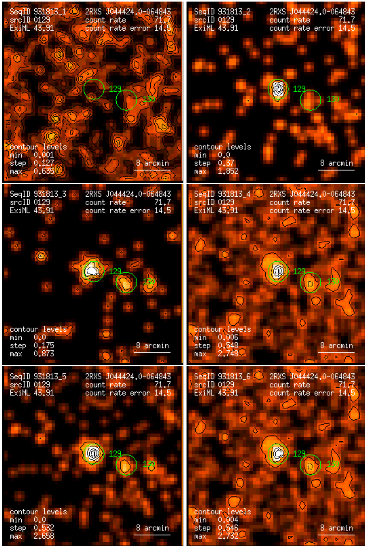
Figure 129: RASS 931813: detection 0129: band rate images, Gaussian filter: (1) PSPC channels 11 – 41, (2) 52 – 90, (3) 91 – 201, (4) 11 – 235, (5) 52 – 201, (6) 11 – 201. Broad band rates in counts/ks. Band rate contour levels in counts/ks/arcmin 2 .
