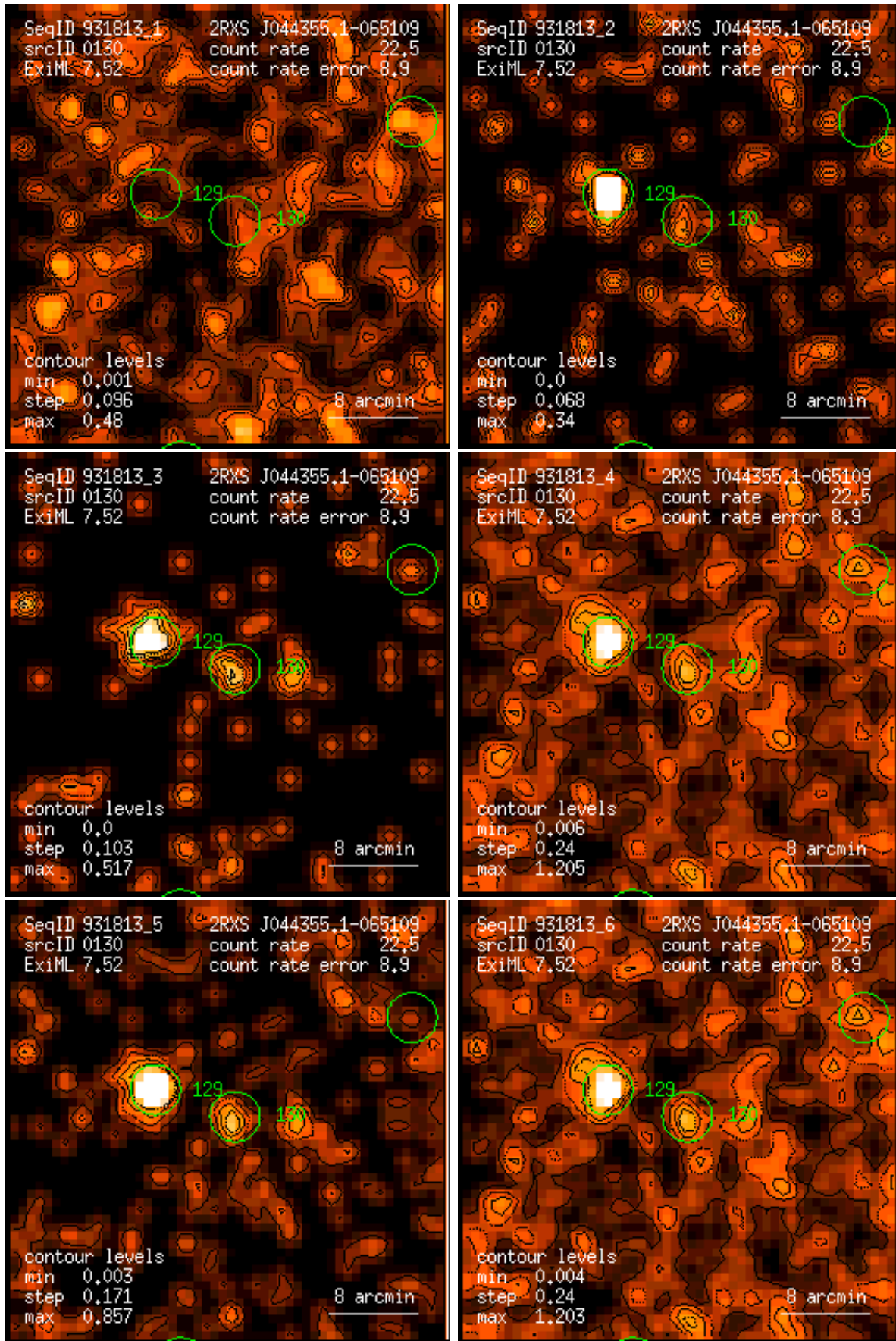
Figure 130: RASS 931813: detection 0130: band rate images, Gaussian filter: (1) PSPC channels 11 – 41, (2) 52 – 90, (3) 91 – 201, (4) 11 – 235, (5) 52 – 201, (6) 11 – 201. Broad band rates in counts/ks. Band rate contour levels in counts/ks/arcmin 2 .
