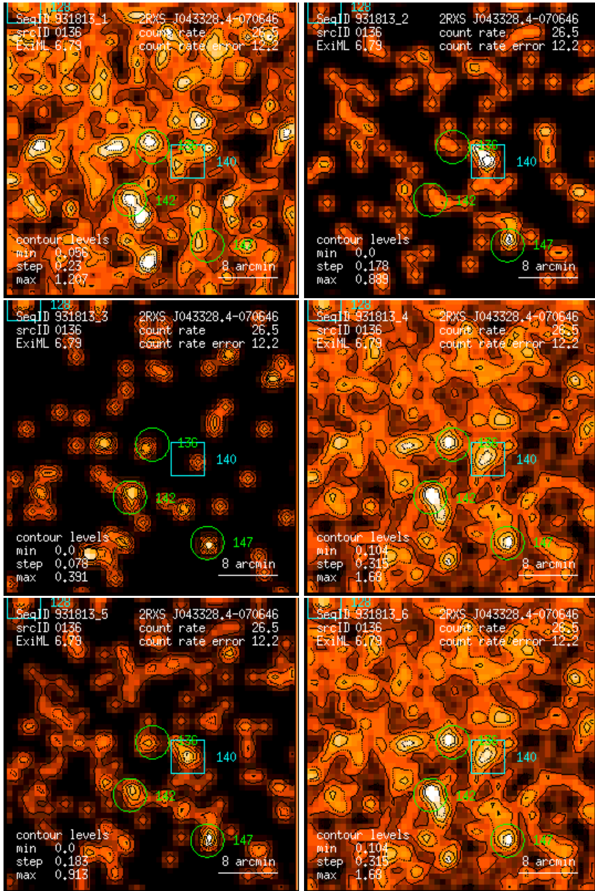
Figure 136: RASS 931813: detection 0136: band rate images, Gaussian filter: (1) PSPC channels 11 – 41, (2) 52 – 90, (3) 91 – 201, (4) 11 – 235, (5) 52 – 201, (6) 11 – 201. Broad band rates in counts/ks. Band rate contour levels in counts/ks/arcmin 2 .
