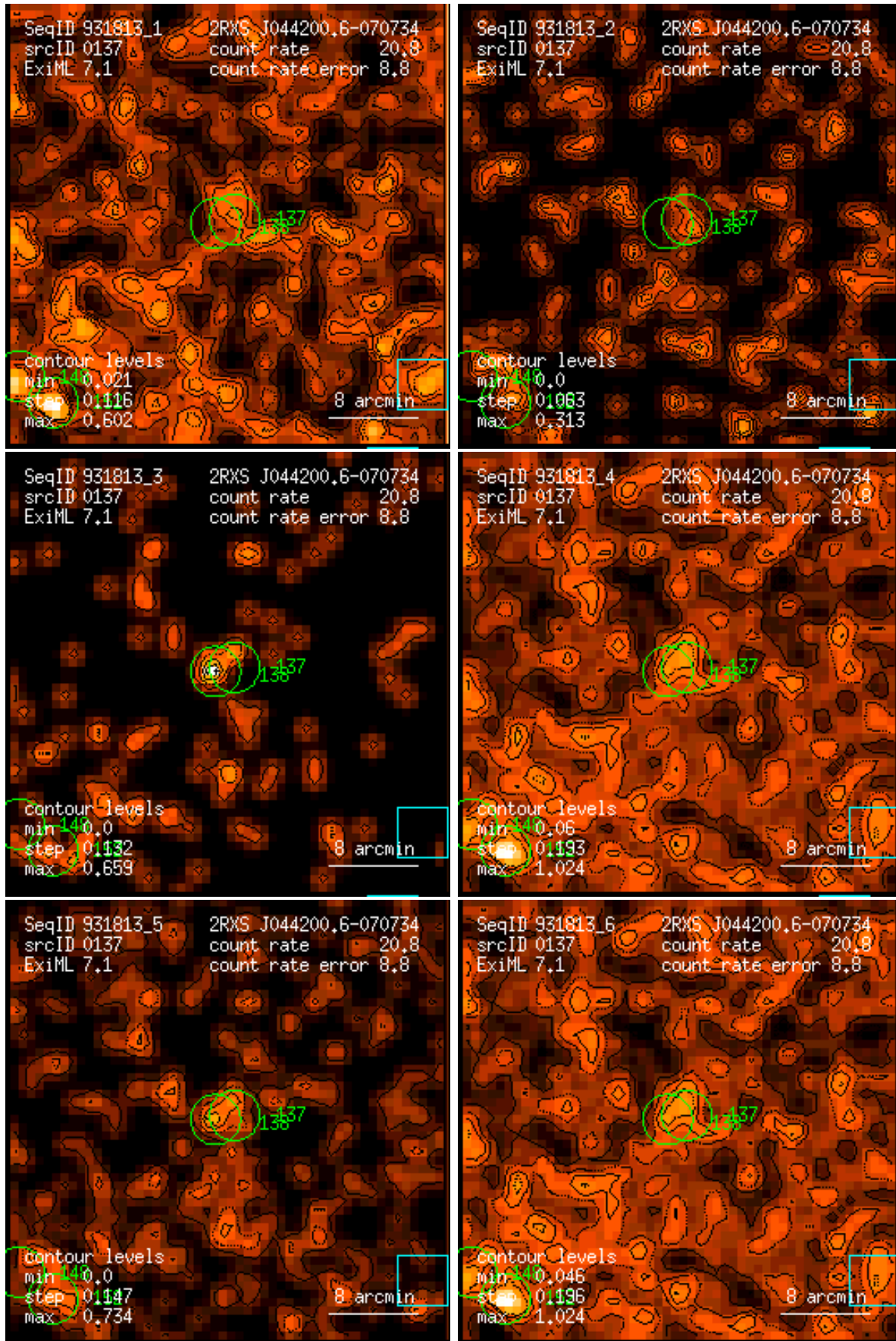
Figure 137: RASS 931813: detection 0137: band rate images, Gaussian filter: (1) PSPC channels 11 – 41, (2) 52 – 90, (3) 91 – 201, (4) 11 – 235, (5) 52 – 201, (6) 11 – 201. Broad band rates in counts/ks. Band rate contour levels in counts/ks/arcmin 2 .
