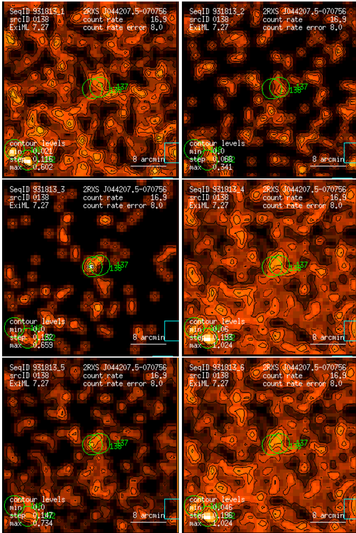
Figure 138: RASS 931813: detection 0138: band rate images, Gaussian filter: (1) PSPC channels 11 – 41, (2) 52 – 90, (3) 91 – 201, (4) 11 – 235, (5) 52 – 201, (6) 11 – 201. Broad band rates in counts/ks. Band rate contour levels in counts/ks/arcmin 2 .
