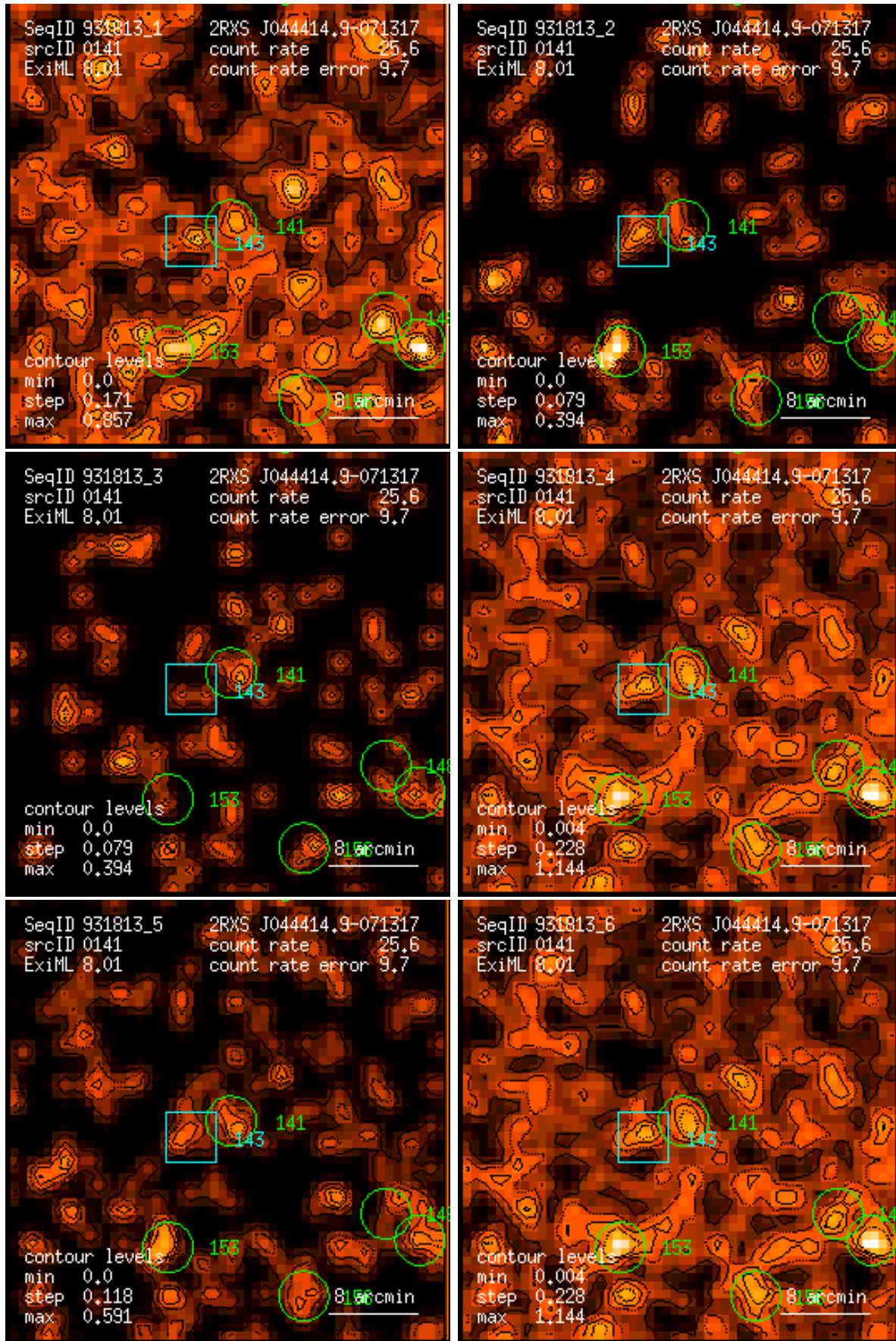
Figure 141: RASS 931813: detection 0141: band rate images, Gaussian filter: (1) PSPC channels 11 – 41, (2) 52 – 90, (3) 91 – 201, (4) 11 – 235, (5) 52 – 201, (6) 11 – 201. Broad band rates in counts/ks. Band rate contour levels in counts/ks/arcmin 2 .
