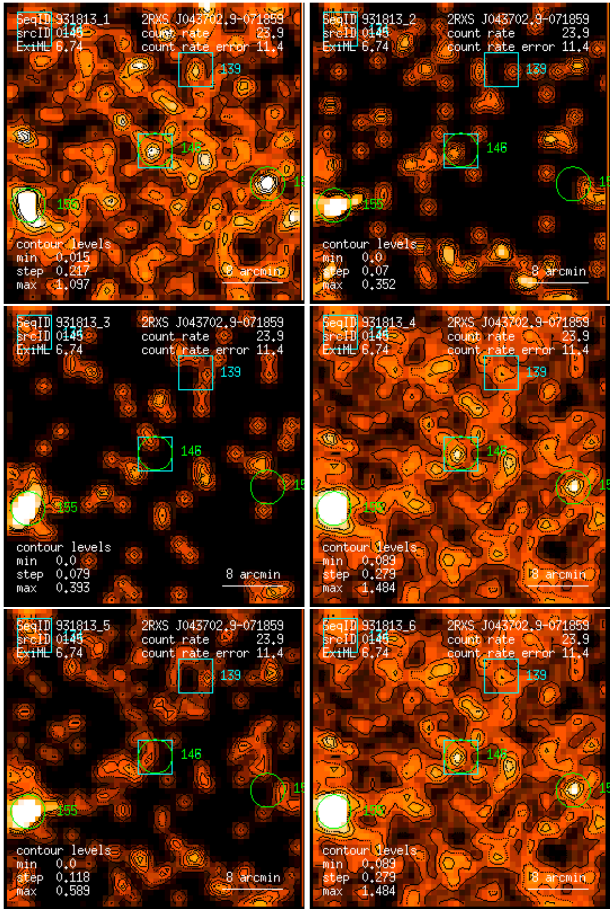
Figure 145: RASS 931813: detection 0145: band rate images, Gaussian filter: (1) PSPC channels 11 – 41, (2) 52 – 90, (3) 91 – 201, (4) 11 – 235, (5) 52 – 201, (6) 11 – 201. Broad band rates in counts/ks. Band rate contour levels in counts/ks/arcmin 2 .
