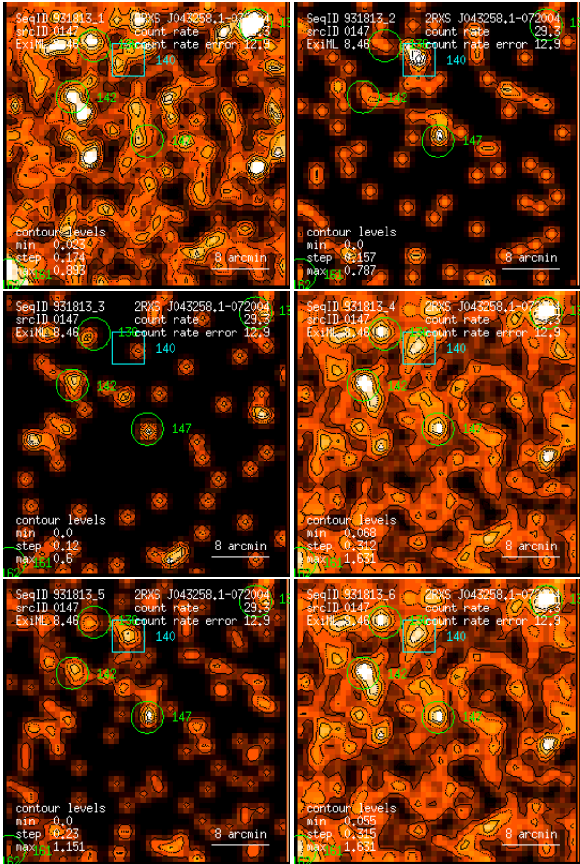
Figure 147: RASS 931813: detection 0147: band rate images, Gaussian filter: (1) PSPC channels 11 – 41, (2) 52 – 90, (3) 91 – 201, (4) 11 – 235, (5) 52 – 201, (6) 11 – 201. Broad band rates in counts/ks. Band rate contour levels in counts/ks/arcmin 2 .
