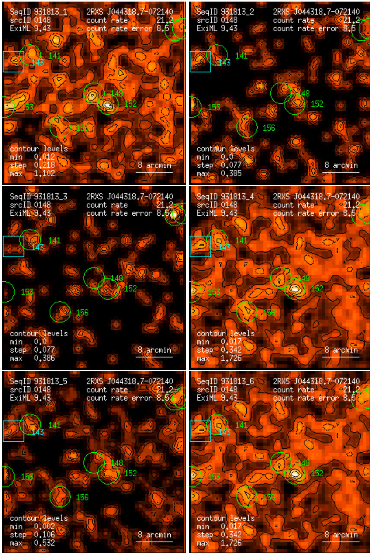
Figure 148: RASS 931813: detection 0148: band rate images, Gaussian filter: (1) PSPC channels 11 – 41, (2) 52 – 90, (3) 91 – 201, (4) 11 – 235, (5) 52 – 201, (6) 11 – 201. Broad band rates in counts/ks. Band rate contour levels in counts/ks/arcmin 2 .
