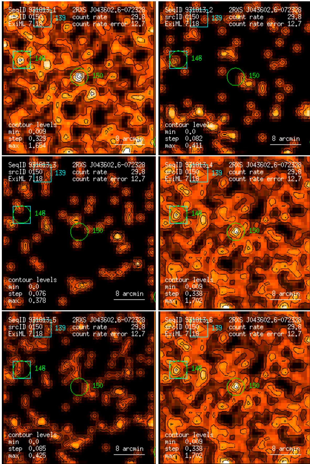
Figure 150: RASS 931813: detection 0150: band rate images, Gaussian filter: (1) PSPC channels 11 – 41, (2) 52 – 90, (3) 91 – 201, (4) 11 – 235, (5) 52 – 201, (6) 11 – 201. Broad band rates in counts/ks. Band rate contour levels in counts/ks/arcmin 2 .
