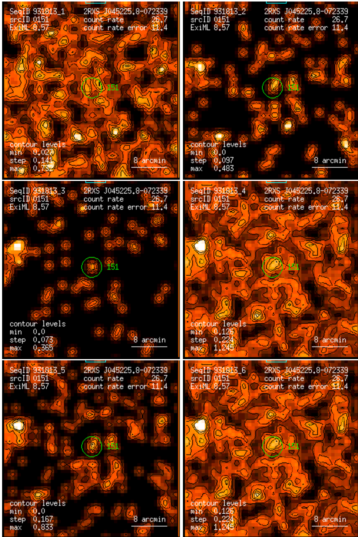
Figure 151: RASS 931813: detection 0151: band rate images, Gaussian filter: (1) PSPC channels 11 – 41, (2) 52 – 90, (3) 91 – 201, (4) 11 – 235, (5) 52 – 201, (6) 11 – 201. Broad band rates in counts/ks. Band rate contour levels in counts/ks/arcmin 2 .
