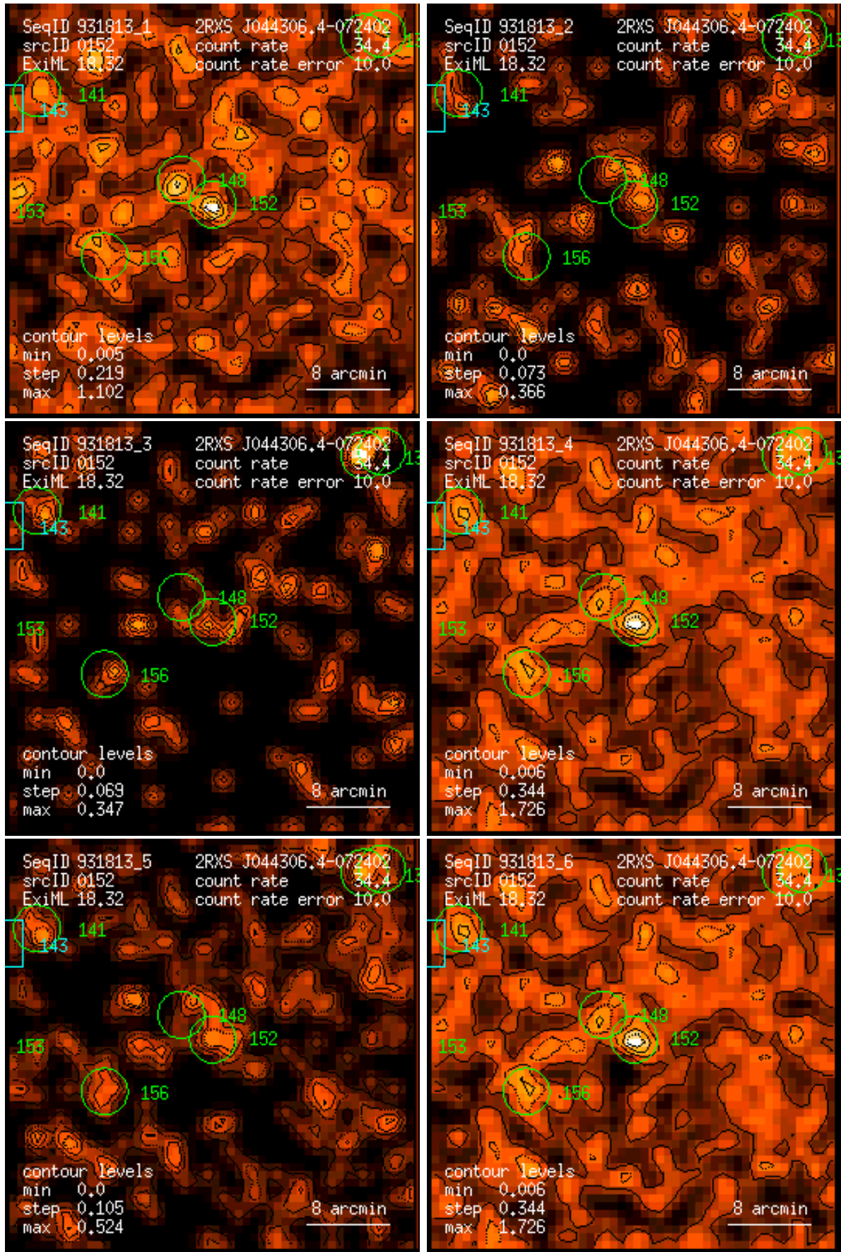
Figure 152: RASS 931813: detection 0152: band rate images, Gaussian filter: (1) PSPC channels 11 – 41, (2) 52 – 90, (3) 91 – 201, (4) 11 – 235, (5) 52 – 201, (6) 11 – 201. Broad band rates in counts/ks. Band rate contour levels in counts/ks/arcmin 2 .
