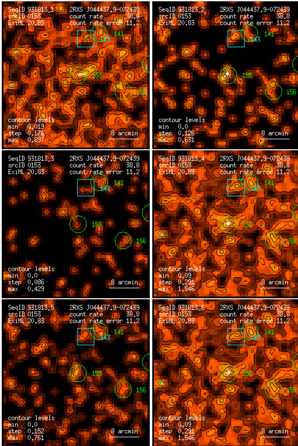
Figure 153: RASS 931813: detection 0153: band rate images, Gaussian filter: (1) PSPC channels 11 – 41, (2) 52 – 90, (3) 91 – 201, (4) 11 – 235, (5) 52 – 201, (6) 11 – 201. Broad band rates in counts/ks. Band rate contour levels in counts/ks/arcmin 2 .
