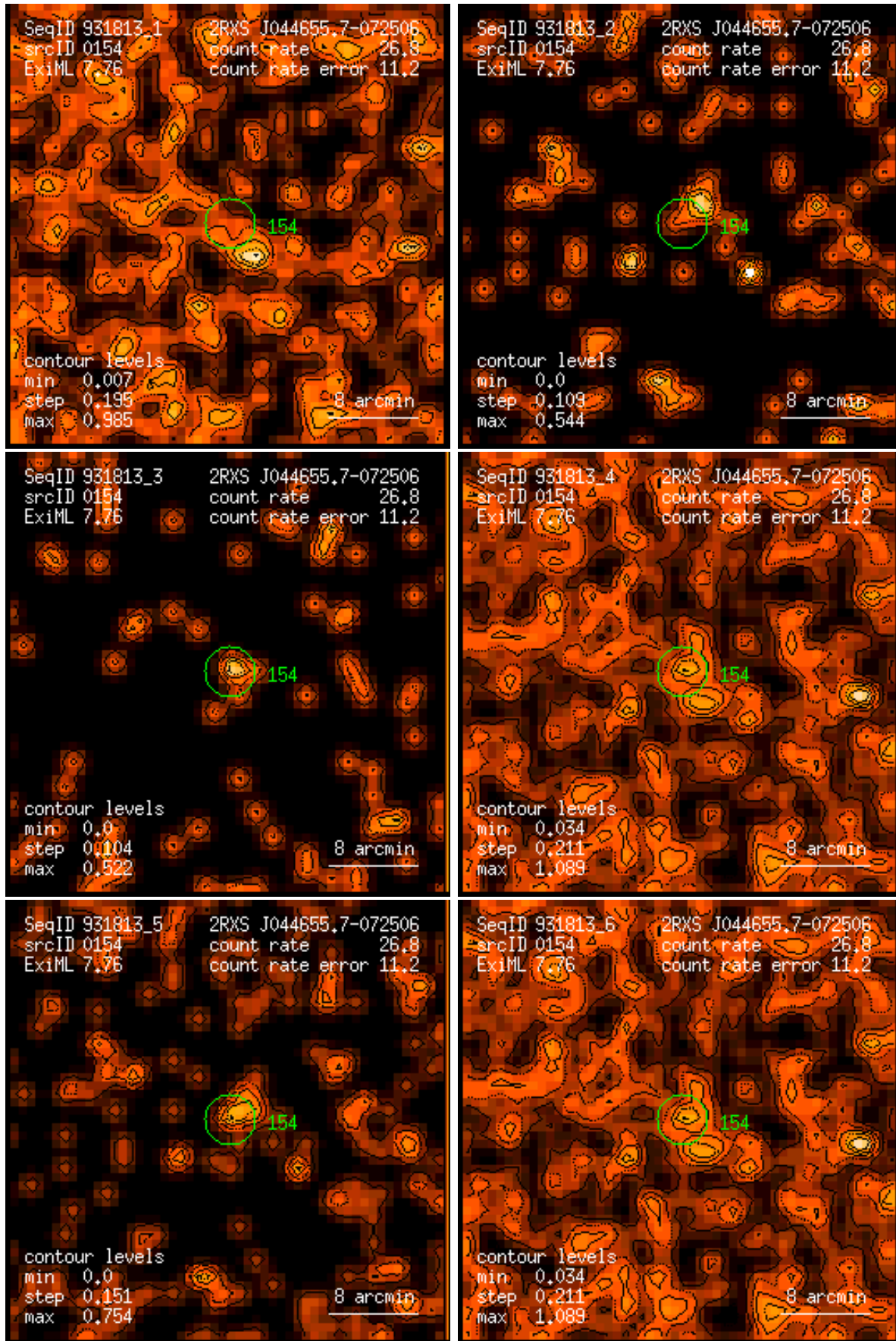
Figure 154: RASS 931813: detection 0154: band rate images, Gaussian filter: (1) PSPC channels 11 – 41, (2) 52 – 90, (3) 91 – 201, (4) 11 – 235, (5) 52 – 201, (6) 11 – 201. Broad band rates in counts/ks. Band rate contour levels in counts/ks/arcmin 2 .
